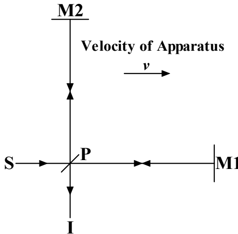
Figure 2. Michelson-Morley Experiment
