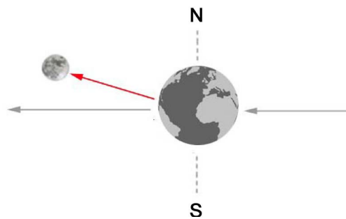
Figure 2. The Moon accelerates the Earth upwards.
