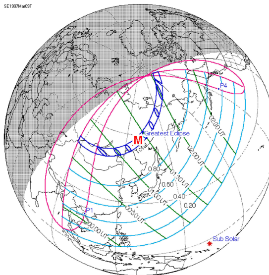
Figure 20. Measurement “M” took place in N-China.
