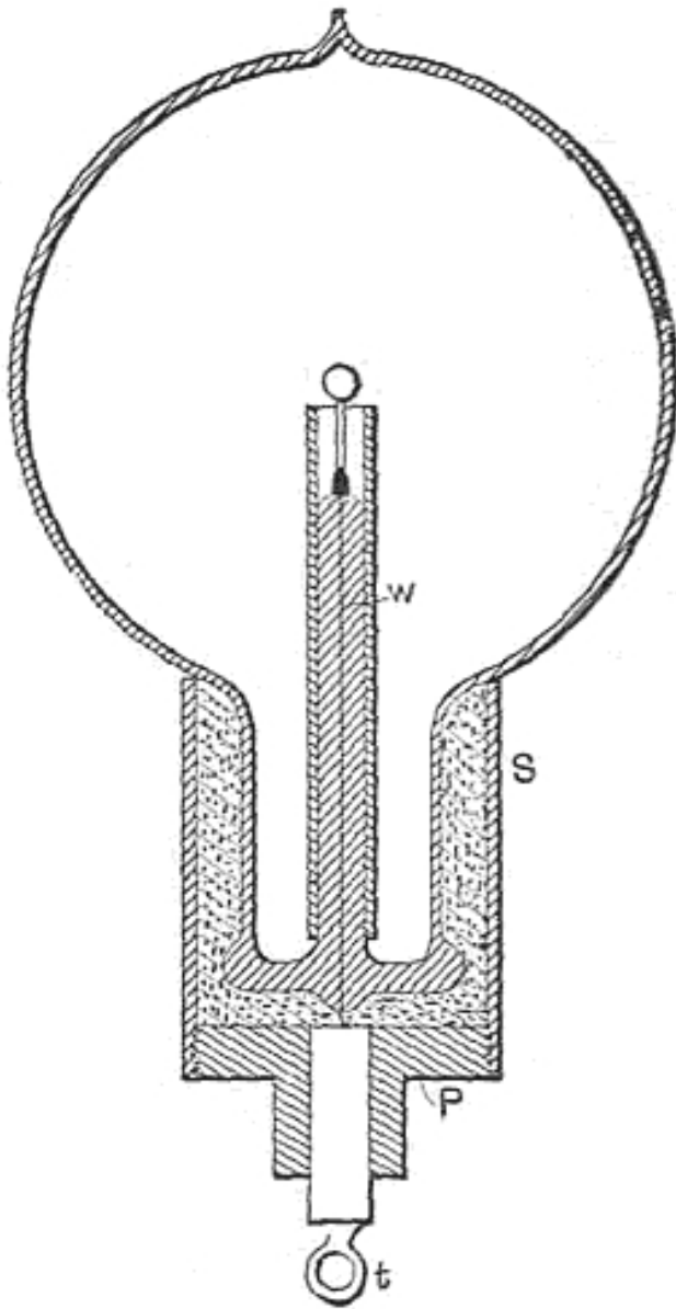
FIG. 19.—IMPROVED BULB WITH SOCKET AND SCREEN.
