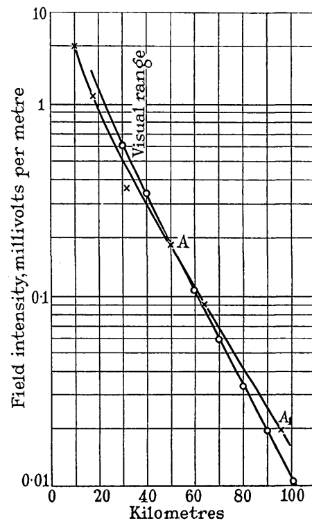
Fig. 31.—Ultra-short-wave diffraction. Results obtained by Jones at 61 megacycles per sec., in transmission from Empire State Building, New York.
