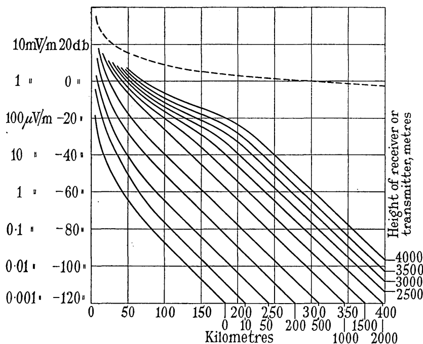
Fig. 23.—Results obtained over land; \lambda = 8 m, \kappa = 5 , \sigma = 10^{-13} , 1 kW radiated.
