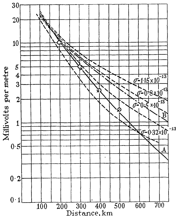
Fig. 35.—Results obtained on Warsaw; \lambda = 1\,400 m, 100 kW radiated.
