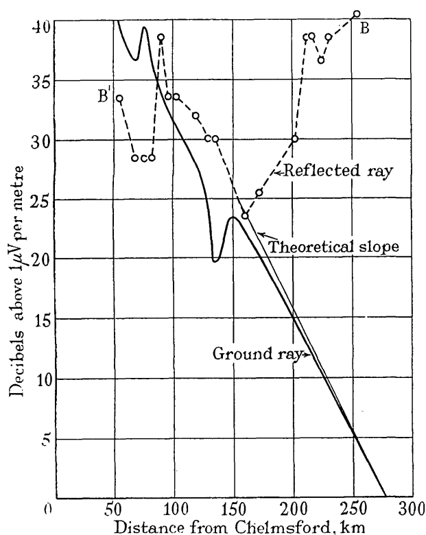
Fig. 32.—Aeroplane test. Results obtained on wavelength of 53.4 m, 1st October, 1935.
