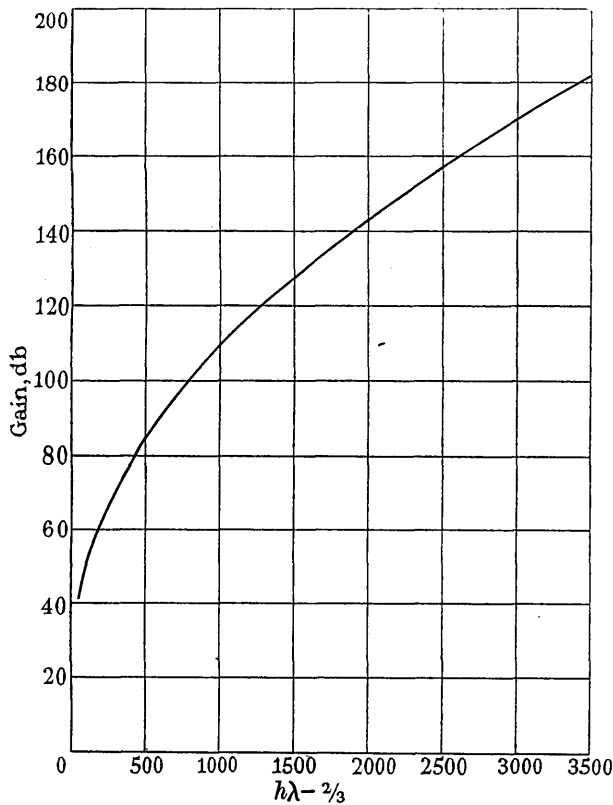
Fig. 3.—Height/gain curves ( h and \lambda in metres).
