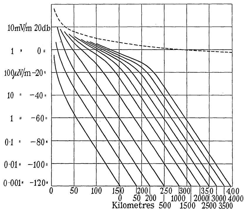
Fig. 7.—Results obtained over sea; \lambda = 2 m, \kappa = 80 , \sigma = 10^{-11} , 1 kW radiated.
