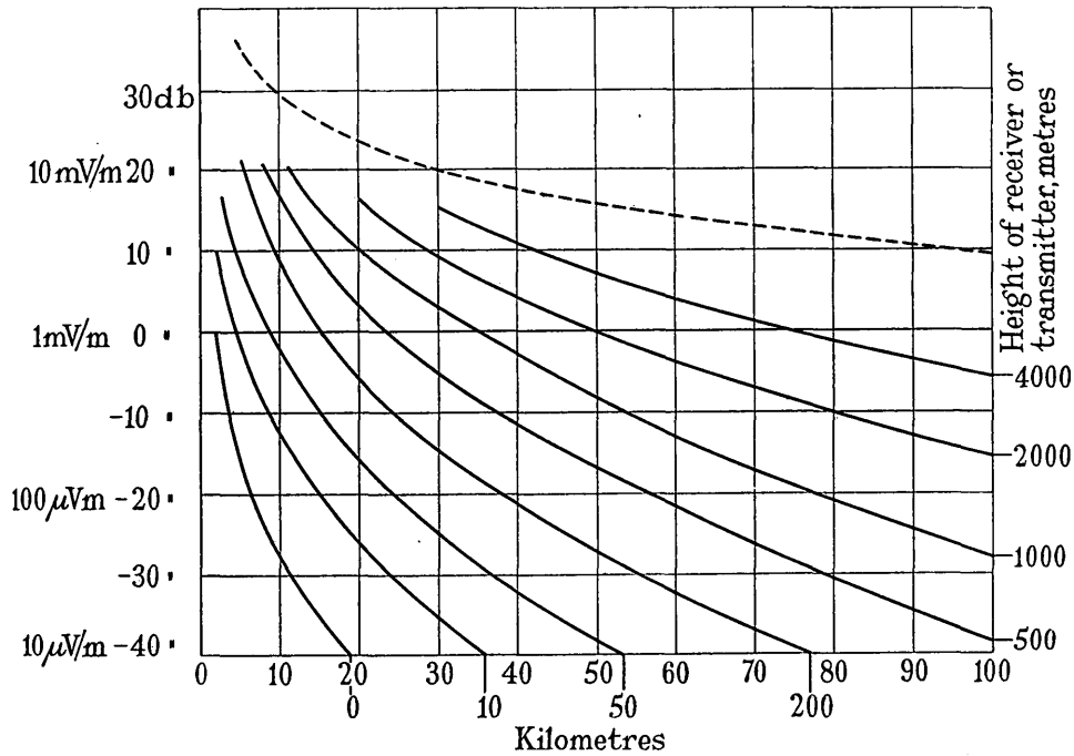
Fig. 24.—Results obtained over land; \lambda = 10 m, \kappa = 5 , \sigma = 10^{-13} , 1 kW radiated.
