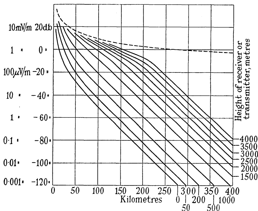
Fig. 13.—Results obtained over sea; \lambda = 8 m, \kappa = 80 , \sigma = 10^{-11} , 1 kW radiated.
