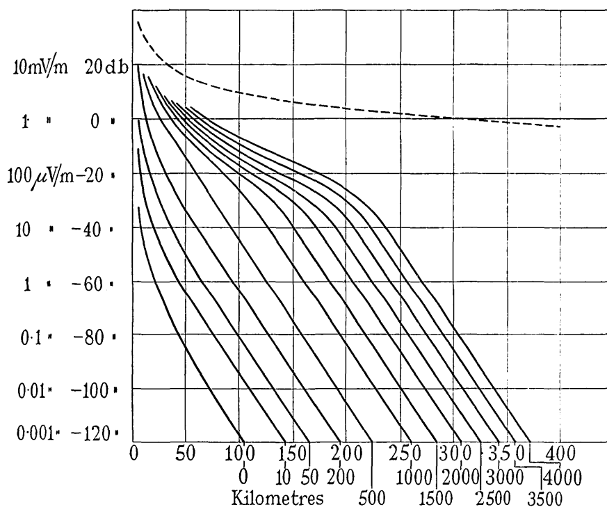
Fig. 17.—Results obtained over land; \lambda = 2 m, \kappa = 5 , \sigma = 10^{-18} , 1 kW radiated. Figures against curves indicate height of receiver or transmitter in metres.
