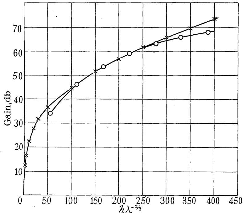
Fig. 38.—Height/gain observations. Results obtained by Trevor and Carter at 44 megacycles per sec., in transmission to distance of 185 km from Empire State Building, New York.
