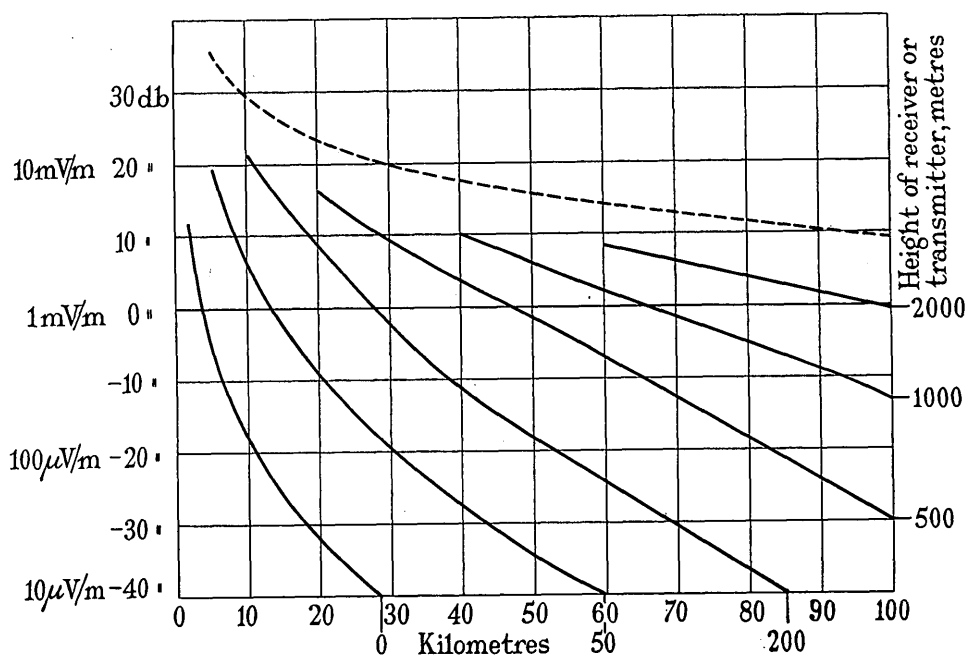
Fig. 6.—Results obtained over sea; \lambda = 2 m, \kappa = 80 , \sigma = 10^{-11} , 1 kW radiated.
