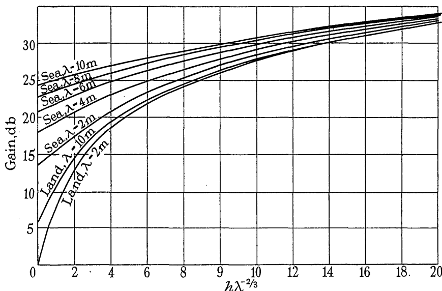
Fig. 5.—Height/gain curves ( h and \lambda in metres).
