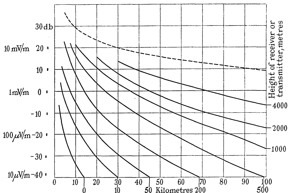
Fig. 20.—Results obtained over land; \lambda = 6 m, \kappa = 5 , \sigma = 10^{-13} , 1 kW radiated.
