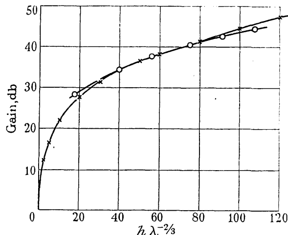
Fig. 36.—Height/gain observations. Results obtained by Jones at 44 megacycles per sec., in transmission to distance of 102 km from Empire State Building, New York. Height of transmitting aerial, 396 m.
