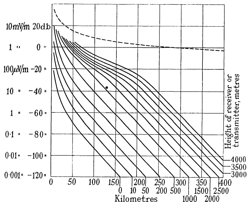
Fig. 21.—Results obtained over land; \lambda = 6 m, \kappa = 5 , \sigma = 10^{-13} , 1 kW radiated.
