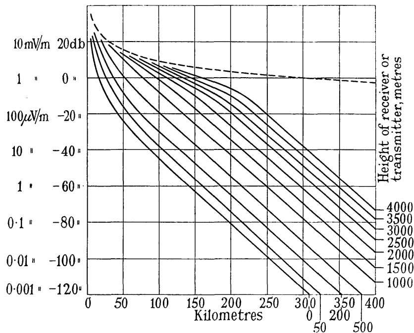
Fig. 15.—Results obtained over sea; \lambda = 10 m, \kappa = 80 , \sigma = 10^{-11} , 1 kW radiated.
