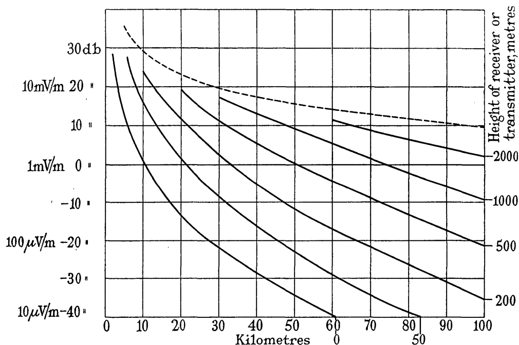
Fig. 10.—Results obtained over sea; \lambda = 6 m, \kappa = 80 , \sigma = 10^{-11} , 1 kW radiated.
