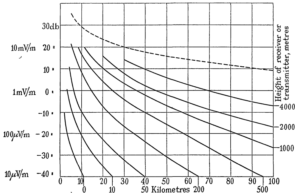
Fig. 18.—Results obtained over land; \lambda = 4 m, \kappa = 5 , \sigma = 10^{-13} , 1 kW radiated.
