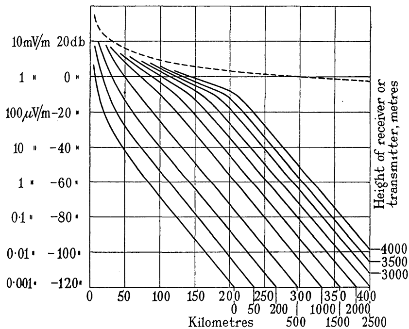
Fig. 9.—Results obtained over sea; \lambda = 4 m, \kappa = 80 , \sigma = 10^{-11} , 1 kW radiated.
