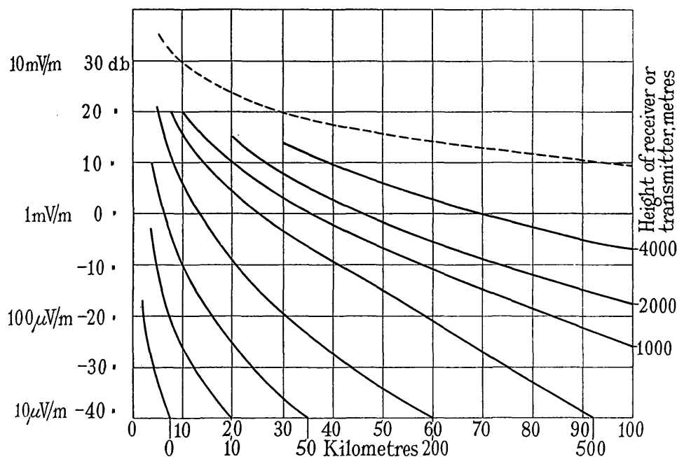
Fig. 16.—Results obtained over land; \lambda = 2 m, \kappa = 5 , \sigma = 10^{-18} , 1 kW radiated.
