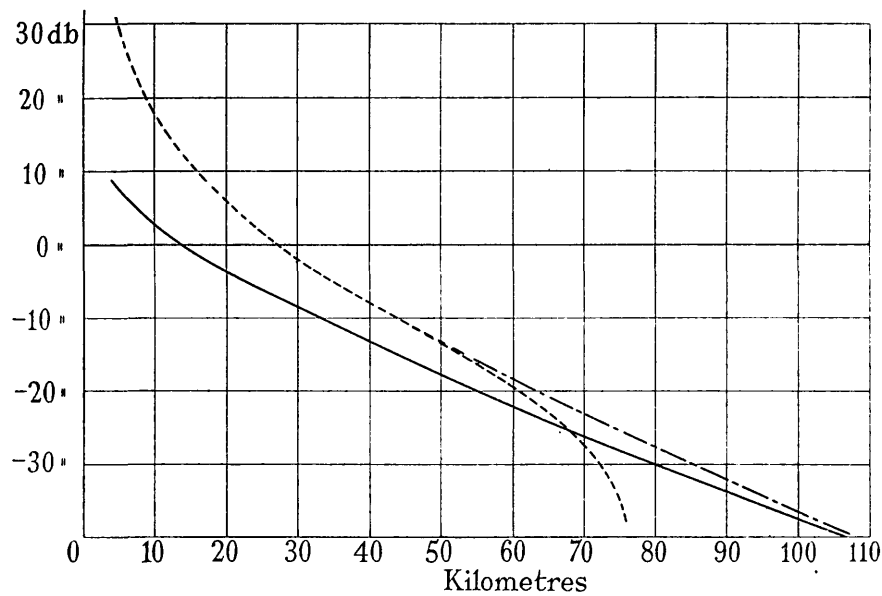
Fig. 29.—Continuity of reciprocal and diffraction values: results obtained over land, \lambda = 10 m, h = 500 m.
