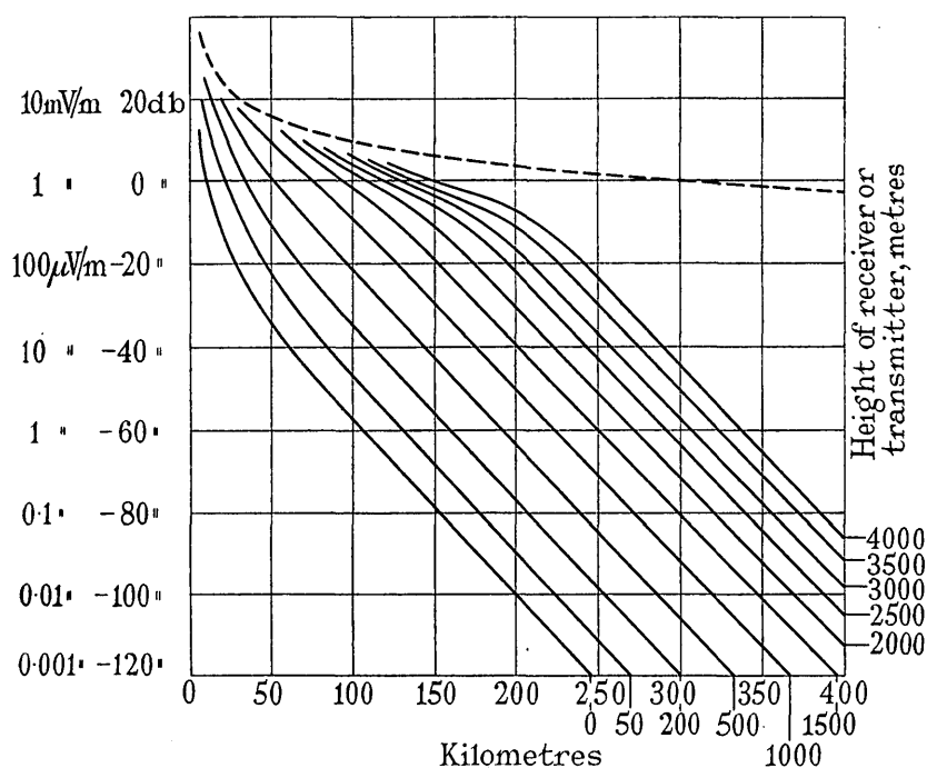
Fig. 11.—Results obtained over sea; \lambda = 6 m, \kappa = 80 , \sigma = 10^{-11} , 1 kW radiated.
