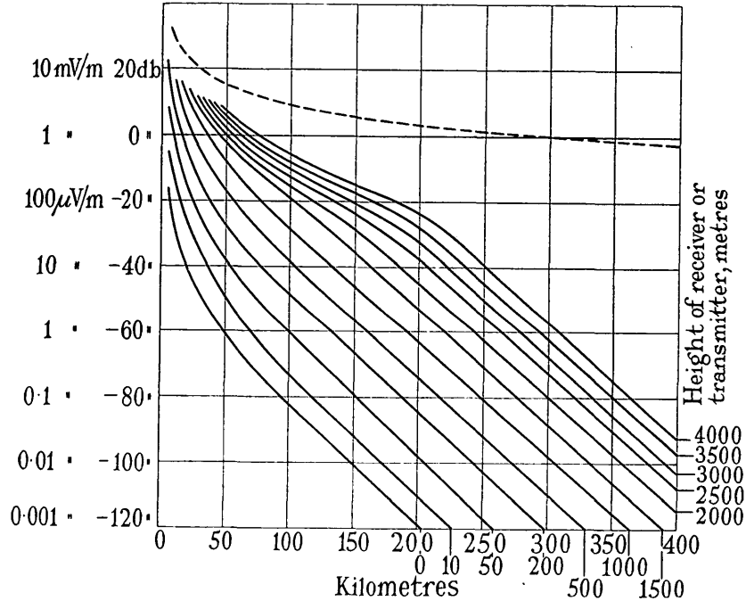
Fig. 25.—Results obtained over land; \lambda = 10 m, \kappa = 5 , \sigma = 10^{-13} , 1 kW radiated.
