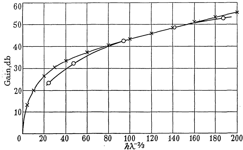
Fig. 37.—Height/gain observations. Results obtained by Trevor and Carter at 34 megacycles per sec., in transmission to distance of 59.6 km from Rocky Point. Height of transmitting aerial, 39 m.
