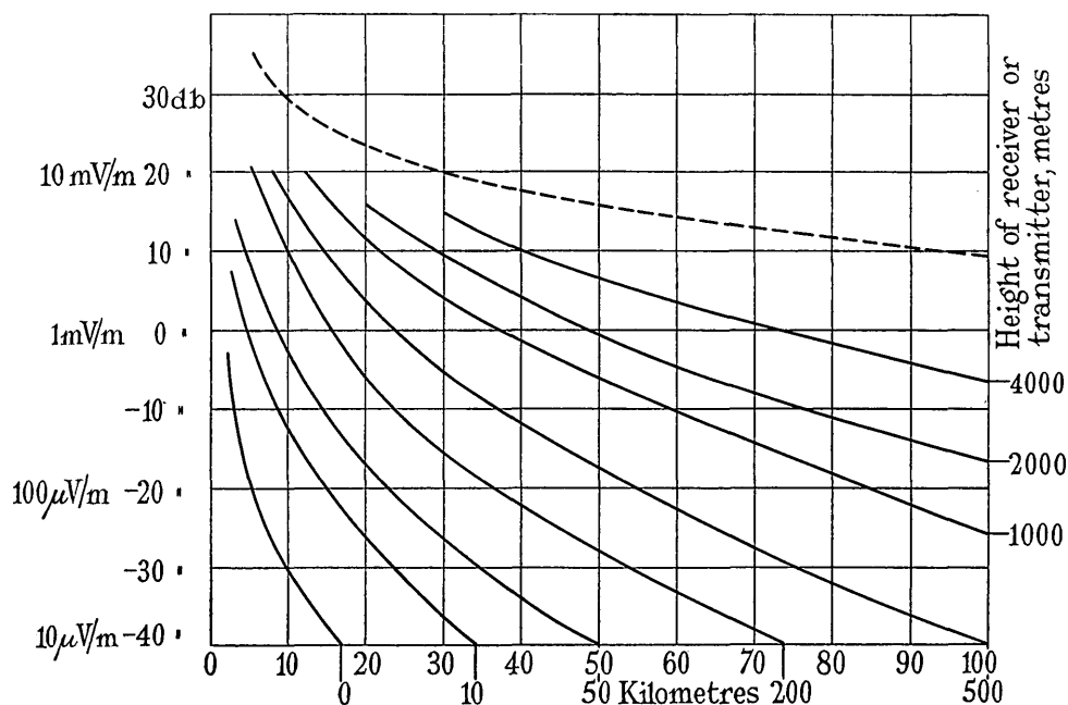
Fig. 22.—Results obtained over land; \lambda = 8 m, \kappa = 5 , \sigma = 10^{-13} , 1 kW radiated.
