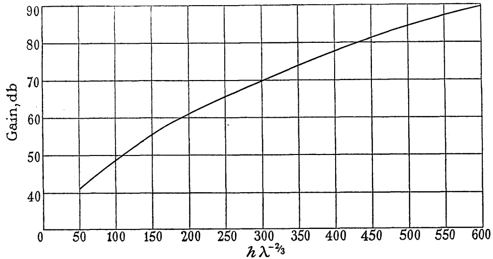
Fig. 2.—Height/gain curves ( h and \lambda in metres).
