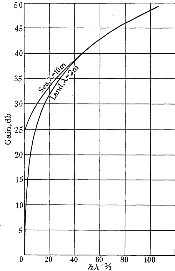
Fig. 4.—Height/gain curves ( h and \lambda in metres).
