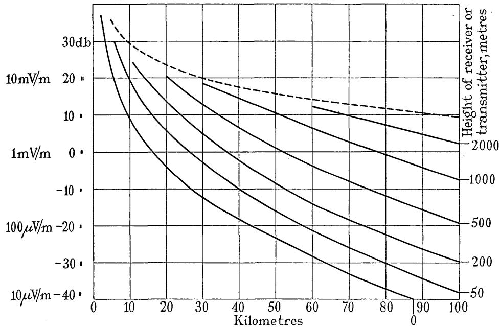
Fig. 14.—Results obtained over sea; \lambda = 10 m, \kappa = 80 , \sigma = 10^{-11} , 1 kW radiated.
