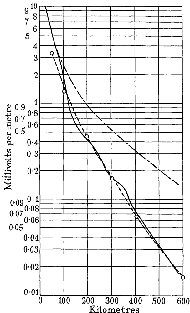
Fig. 33.—Aeroplane test. Results obtained on wavelength of 950 m.
