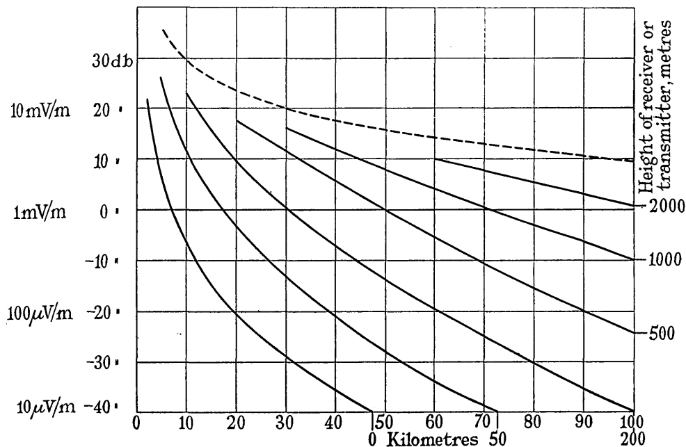
Fig. 8.—Results obtained over sea; \lambda = 4 m, \kappa = 80 , \sigma = 10^{-11} , 1 kW radiated.
