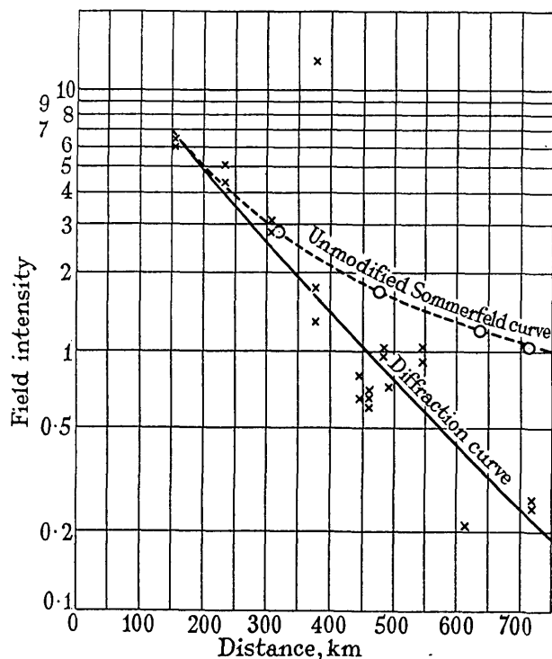
Fig. 34.—Daylight field strength of Daventry 5XX. Results obtained at midday, July, 1931; \lambda = 1\,550 m; normal power (25 kW).
