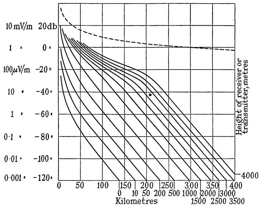
Fig. 19.—Results obtained over land; \lambda = 4 m, \kappa = 5 , \sigma = 10^{-13} , 1 kW radiated.
