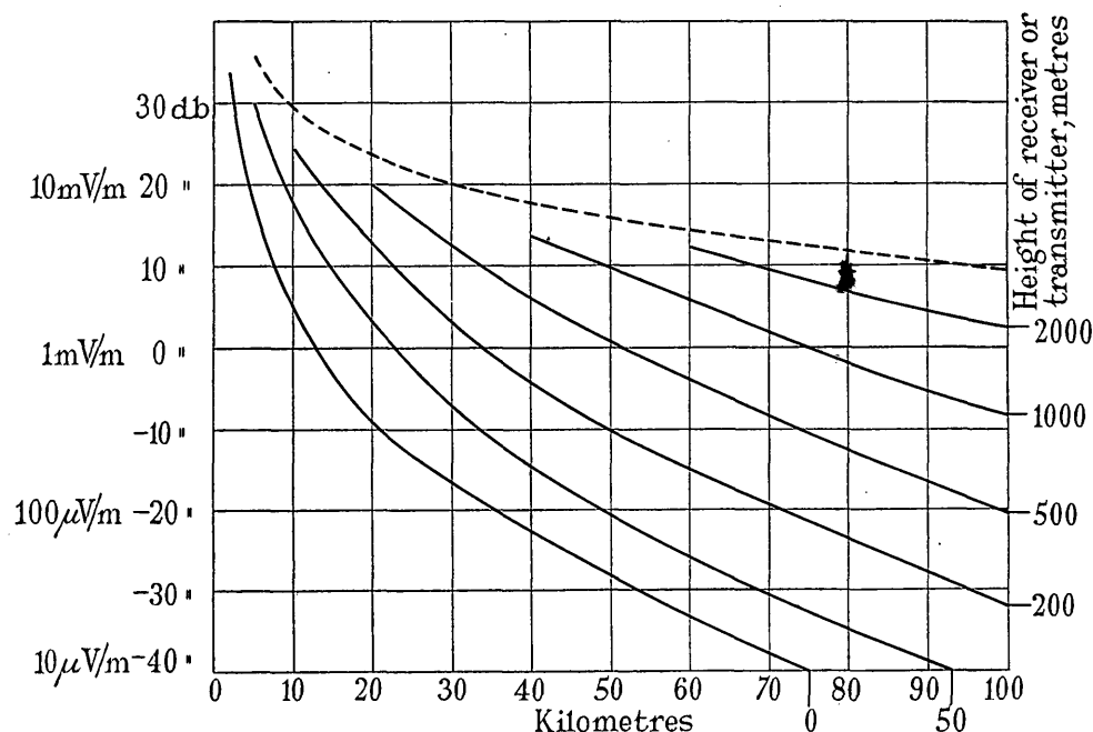
Fig. 12.—Results obtained over sea; \lambda = 8 m, \kappa = 80 , \sigma = 10^{-11} , 1 kW radiated.
