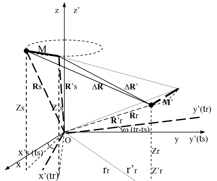
Fig.7 The Sagnac correction in ECEF
