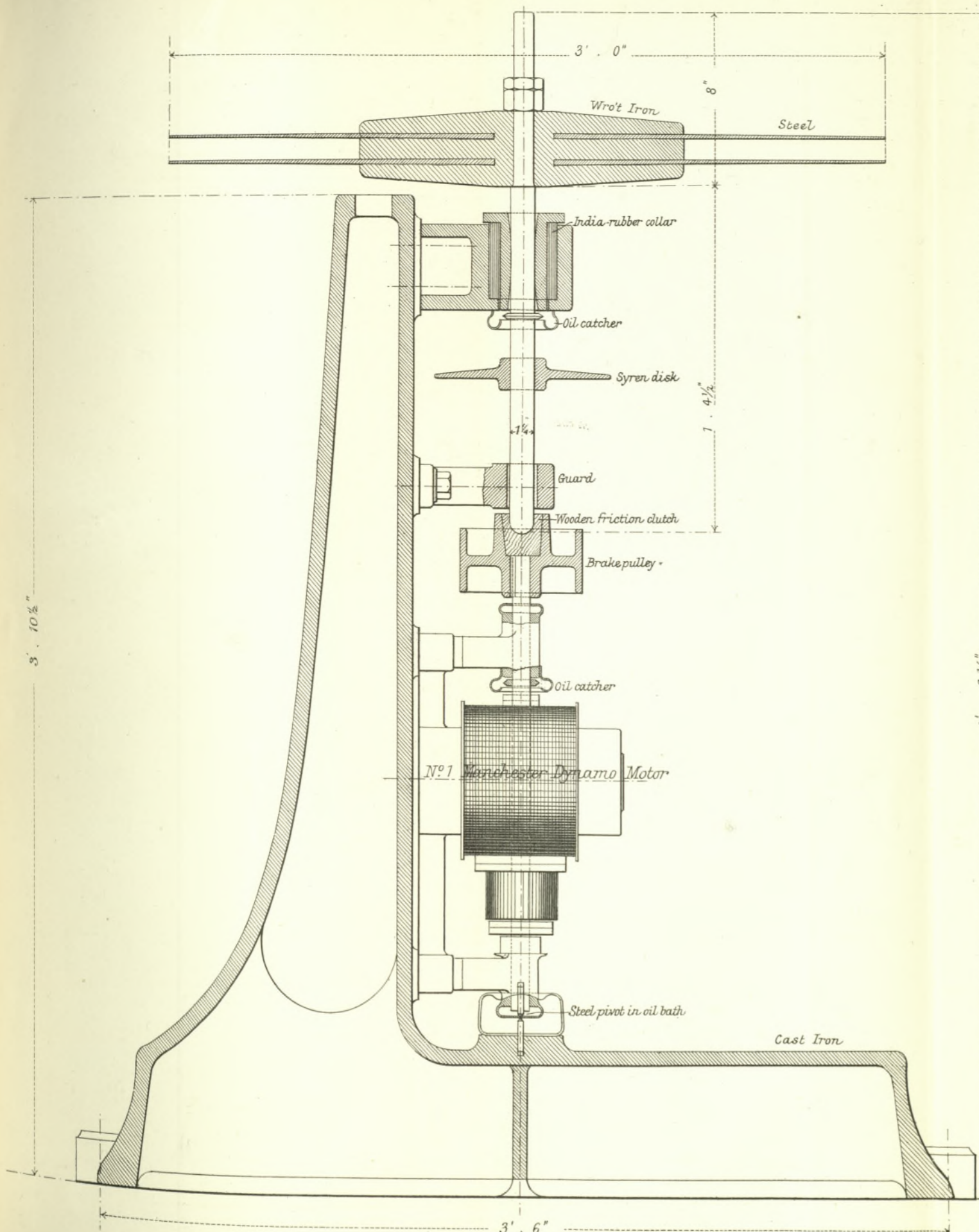
EXPERIMENTAL WHIRLING MACHINE.
