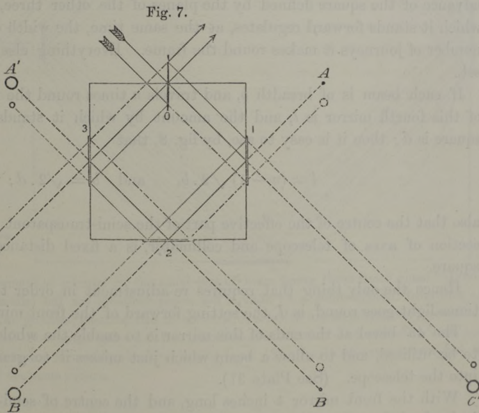
Diagram showing images in simplest case, with three mirrors, and beam going only once round optical square. The points to be imaged are the splitting points on semi-transparent mirror O. Two such points are shown, one imaged by a dot, the other by a ring. A represents the pair of images in first mirror for the transmitted ray; B the image of these in second mirror; C the image in mirror 3. Dashed letters mark the corresponding images for the reflected ray; and the final function of the semi-transparent mirror is to make C' coincide with C so as to give interference.
