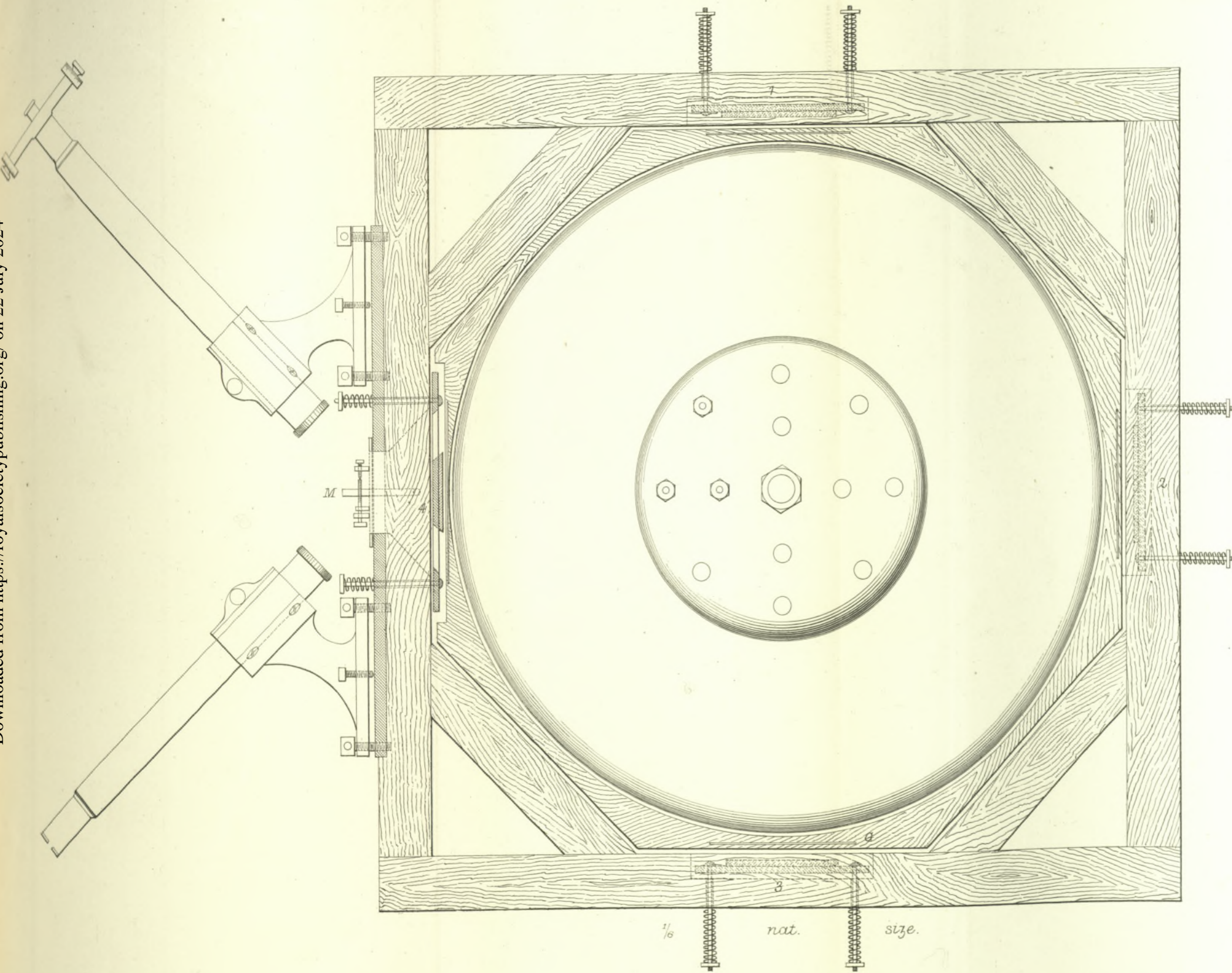
Plan of optical frame with steel disk in position, and glazed drum to isolate them from the frame. G represents one of the panes of optical glass. Supports of telescope and collimator also shewn, and part of the fixing of the four mirrors 1.2.3.4., three of them let into recesses in the wooden frame, each mirror held by a brass plate supported by three finely cut screws against which it is pressed by the spring-bolts shewn. M is the semi-transparent mirror.
