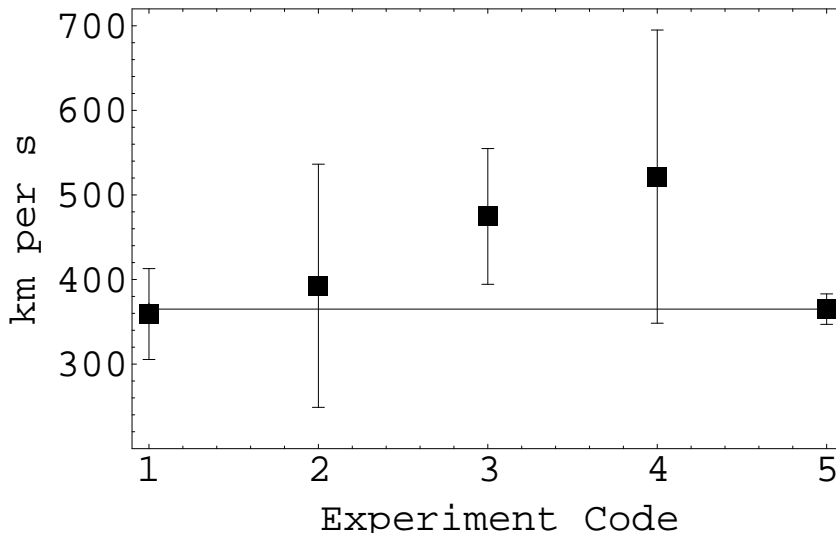
Figure 2: Speeds v_{QF} in km/s determined from various Michelson-Morley experiments: (1) Michelson-Morley (noon observations) [2], (2) Michelson-Morley experiments ( 18^h observations) [2], (3) Miller, Mt. Wilson [11, 12], (4) Illingworth [14], and finally in (5) the speed from the COBE satellite observation of the CBR microwave spectrum dipole term [9]. The results (1)-(4) are not corrected for the \pm 30\text{km/s} of the orbital motion of the earth about the sun, though this correction was made, as well as that for the satellite orbital speed, in the case of (5). The agreement between the Michelson-Morley result in (1) and the COBE result in (5) is striking. The horizontal line at v = 365\text{km/s} is to aid comparisons with the COBE data.
