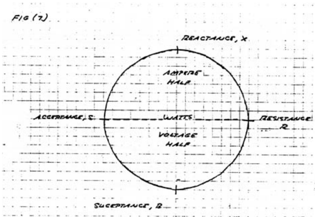
ALTERNATING CURRENTS VERSOR DIAGRAM EMF AND DISPLACEMENT CURRENT
