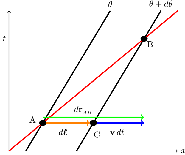
Figure 5: Space-time diagram describing the travel of a nodal point across an infinitesimal fiber's segment d\theta . The diagram shows the projections of all 3D vectors in one direction. The two parallel black lines are the world-lines of the two segment's edges. The red line is the world-line of the node. The lines intersect at the events A and B when the node enters and leaves the segment. Also shown are the vectors \mathbf{e}d\theta = d\boldsymbol{\ell} , d\mathbf{r}_{AB} and \mathbf{v}dt which participate in Eq. (17).
