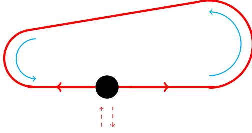
Figure 3: An example of a Wang interferometer: The optical fiber shown as the red curve moves in the direction marked by the cyan arrows. The black dot represents the co-moving beam-splitter and the two dashed red arrows the light source and detector. The counter-propagating light-beams share a common path and are marked by red arrows.
