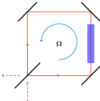
Figure 1: The Sagnac interferometer rotates as a rigid body in the lab with angular velocity \Omega . The beam splitter is at the bottom left corner. The two counter-propagating beams are marked by red arrows; One beam propagates with and the other against the rotation. The optical path may contain co-moving dielectric medium shown as a blue rectangle. The incoming source and outgoing signal are marked by dashed arrows.
