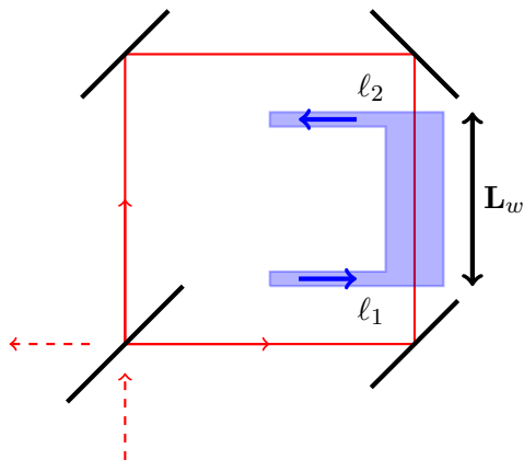
Figure 2: Schematic Fizeau interferometer. The three mirrors and beams splitter are at rest in the lab. The two counter-propagating beams are denoted by the red arrows. Fluid, say water, is flowing in one arm of the interferometer so one beam is moving against the flow and one with the flow.
