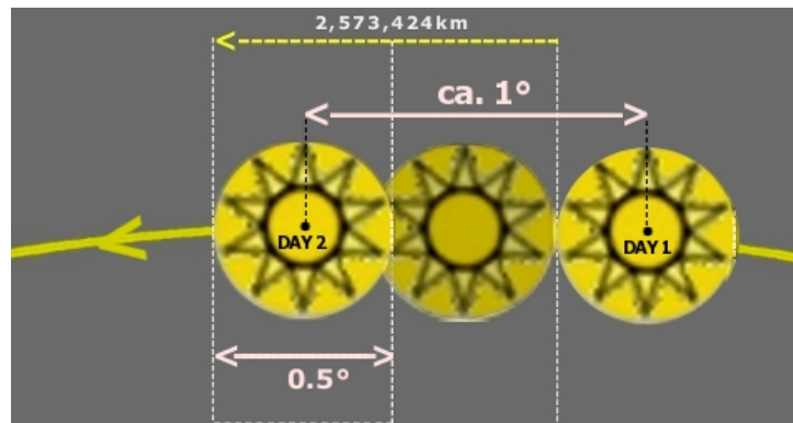
Fig. 12.3 At the speed of 107226 km/h, the Sun will cover 2 573 424 km each day; almost twice its own diameter.
