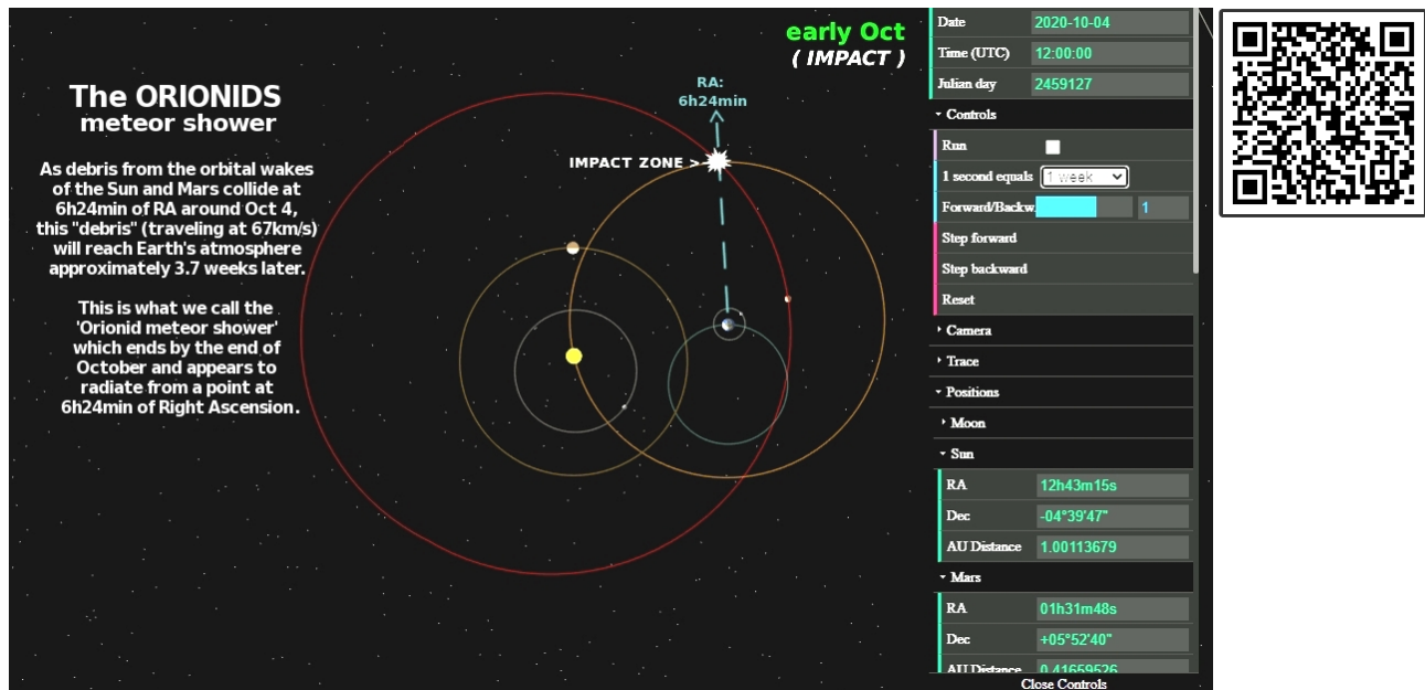
Fig. 15.7 Genesis of the Orionid meteor shower. To animate the graphic, scan the QR code with a smart phone.
