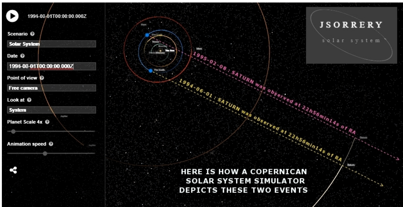
Fig. 17.7 Screenshot from the heliocentric JS orrery.
