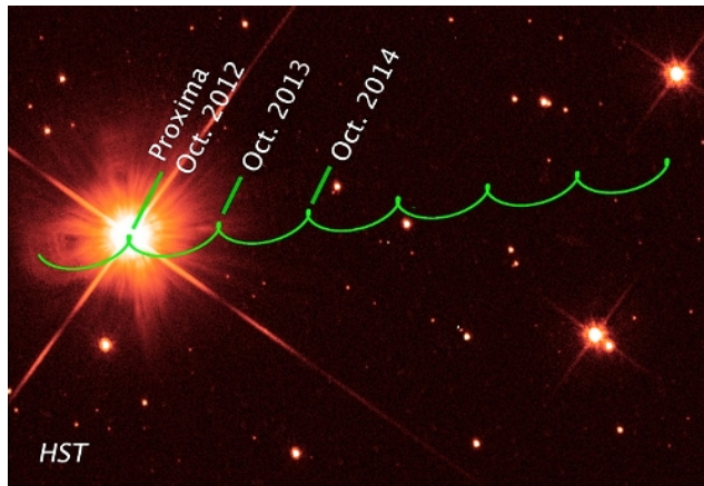
Fig. 21.5 Credited to NASA, this illustration features the following caption: “ The looping action is the result of the Earth’s motion around the Sun. ” Source: Hunting for planets around Proxima Centauri, by D. Dickinson [3].
