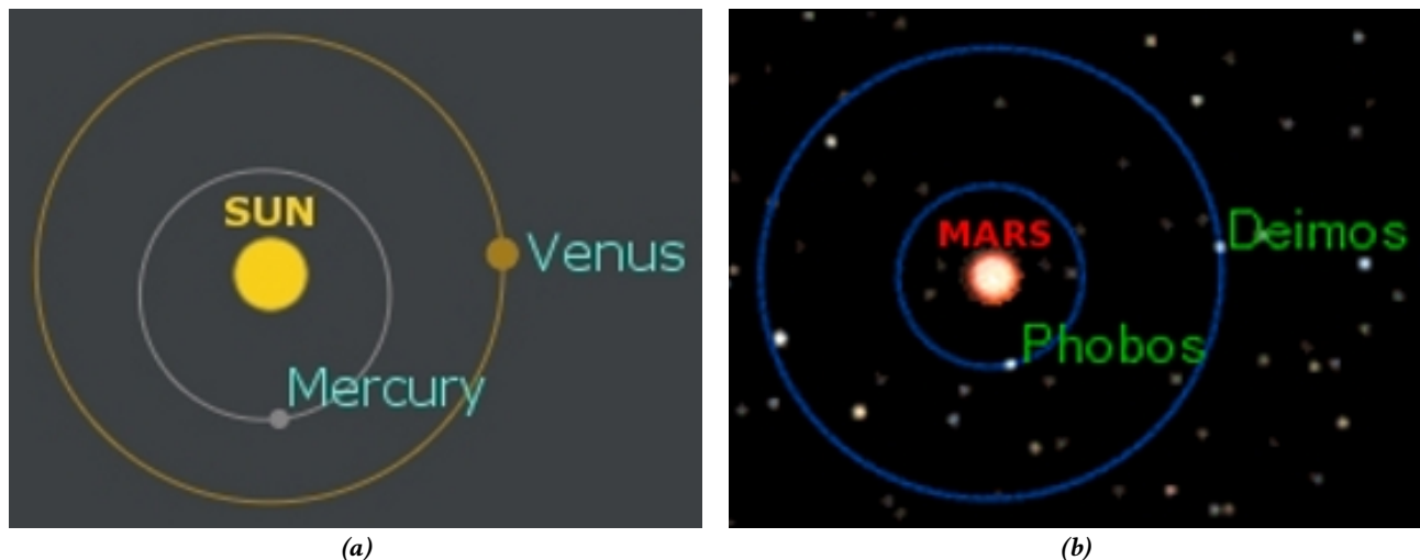
Fig. 3.9 The moons of the Sun and Mars: Mercury and Venus, and Phobos and Deimos.
