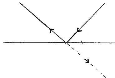
Fig. 4. Professor Hastings's diagram of the path of light at the interface.
