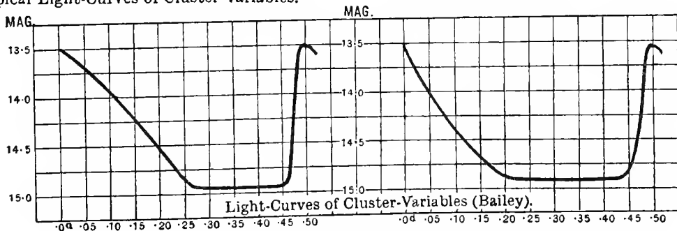
Light curves of Cluster-variables, and of SS Cygni, and S Arae, which are essentially similar.
