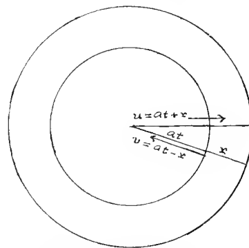
Fig. 16. Illustrating the Wave Theory of Poisson , as in reflected Light.
