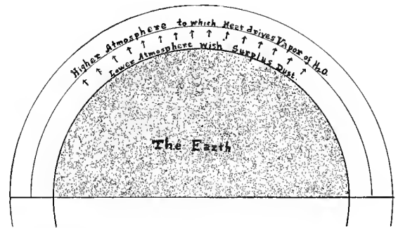
Fig. 10. Illustration of the escape of water vapor, molecular weight 18, to the higher regions of the atmosphere, which is relatively so free from dust, and condensation therefore so difficult, that when a drought in a large inland country once becomes established, it is apt to be prolonged till the larger seasonal changes produce such commotion in the earth's atmosphere as to bring on rain.
