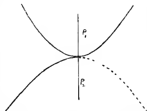
Fig. 19. Sketch of the radii of curvature for a minimal surface, \rho_1 + \rho_2 = 1/R_1 + 1/R_2 = 0 .
