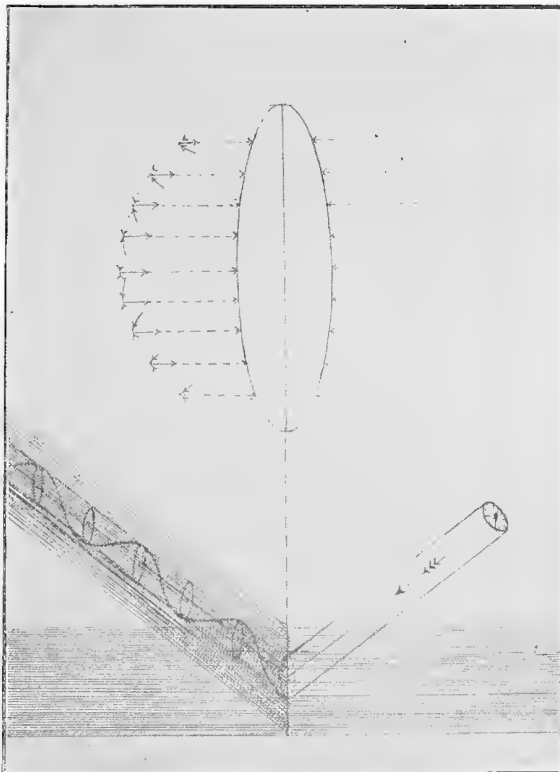
Fig. 6. Illustration of the restriction of free vibrations when the wave motion is suddenly resisted at the boundary of a solid body. Owing to the resistance to one side of the ray the beam of light is flattened like a reflected stream of water, and thenceforth becomes polarized, vibrating with greatest freedom and largest amplitude in the plane perpendicular to the plane of polarization, as held by Fresnel.
