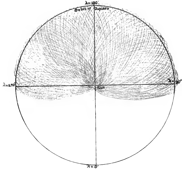
Fig. 7. Illustration of the unsymmetrical distribution of comet orbits and meteoric swarms about Jupiter's orbit, which authorizes the use of the term \Delta\pi(\sigma_0/\sigma_1)\sin[\beta-\alpha(t-t_0)] in the formula for the sunspot periodicity.
