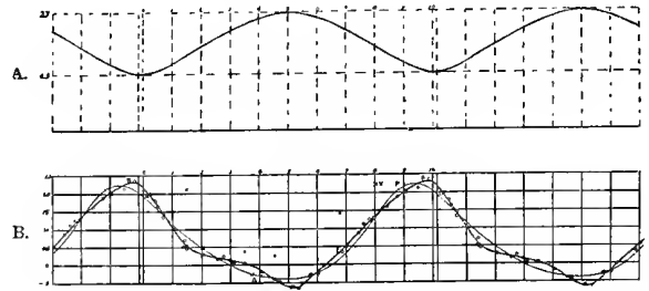
Curves representing the Variations (A) in Light, (B) in Radial Velocity of ζ Geminorum (Campbell).
