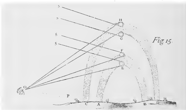
Fig. 3. General outline of the theory of the rainbow given in Newton's Optics, 1704.
