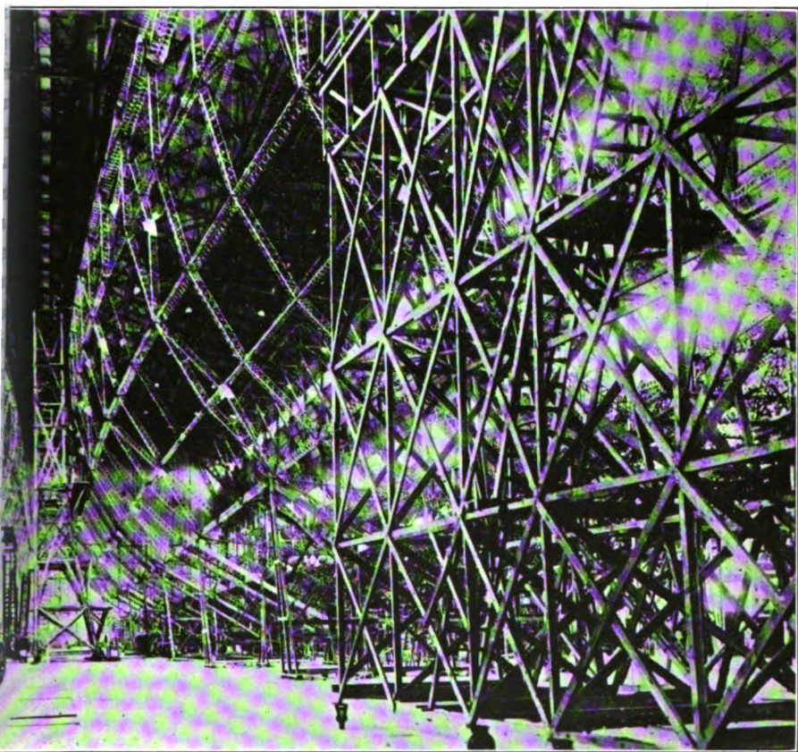
FIG. 16.—ZR-2 in Process of Erection.
