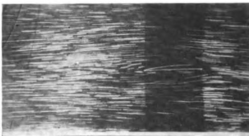
FIG. 17.—Flow Over a Wing at Small Angle of Incidence. (The Wing is Shown in Section. The Dark Vertical Band is a Shadow.)
