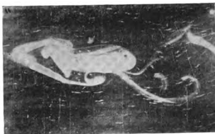
FIG. 19.—Eddy in Wake of Wing. Two Eddies Begin as Small Whirlpools. Flow is from the Left Visible by Condensed Milk in Water.
