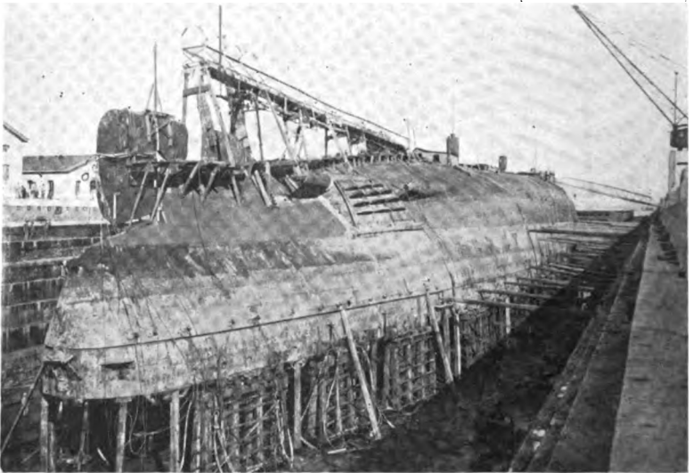
VESSEL IN DRY DOCK SHOWING SUPPORTS.
