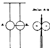
FIG. 16.—Showing How Two Balls Are Sucked Together by a Blast of Air Passing Between Them.
