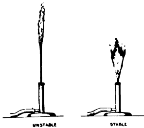
FIG. 6.—Sensitive Flame Before and After Shock Caused by a Whistle of High Pitch.
