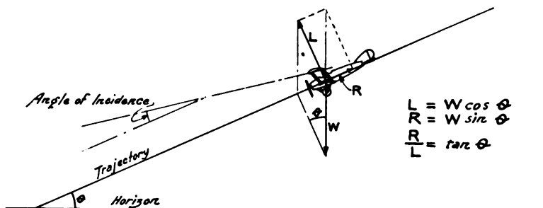
FIG. 22.—Balance of Forces in a Glide.
