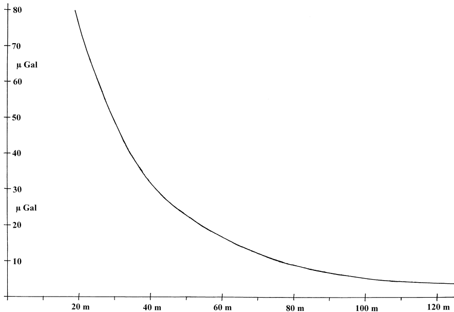
Fig. 5. The effect of a building, 27 m square, 100 m high, 25 \times 10^6 kg mass and average density of 340 \text{ kg/m}^3 , with distance from the centre of the building in \mu\text{Gal} , calculated as a Hammer zone compartment of suitable dimensions and density.
