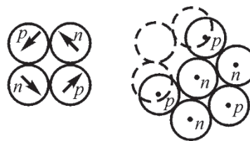
Fig. 6.18. Structure of core ^{10}_5\text{B}
