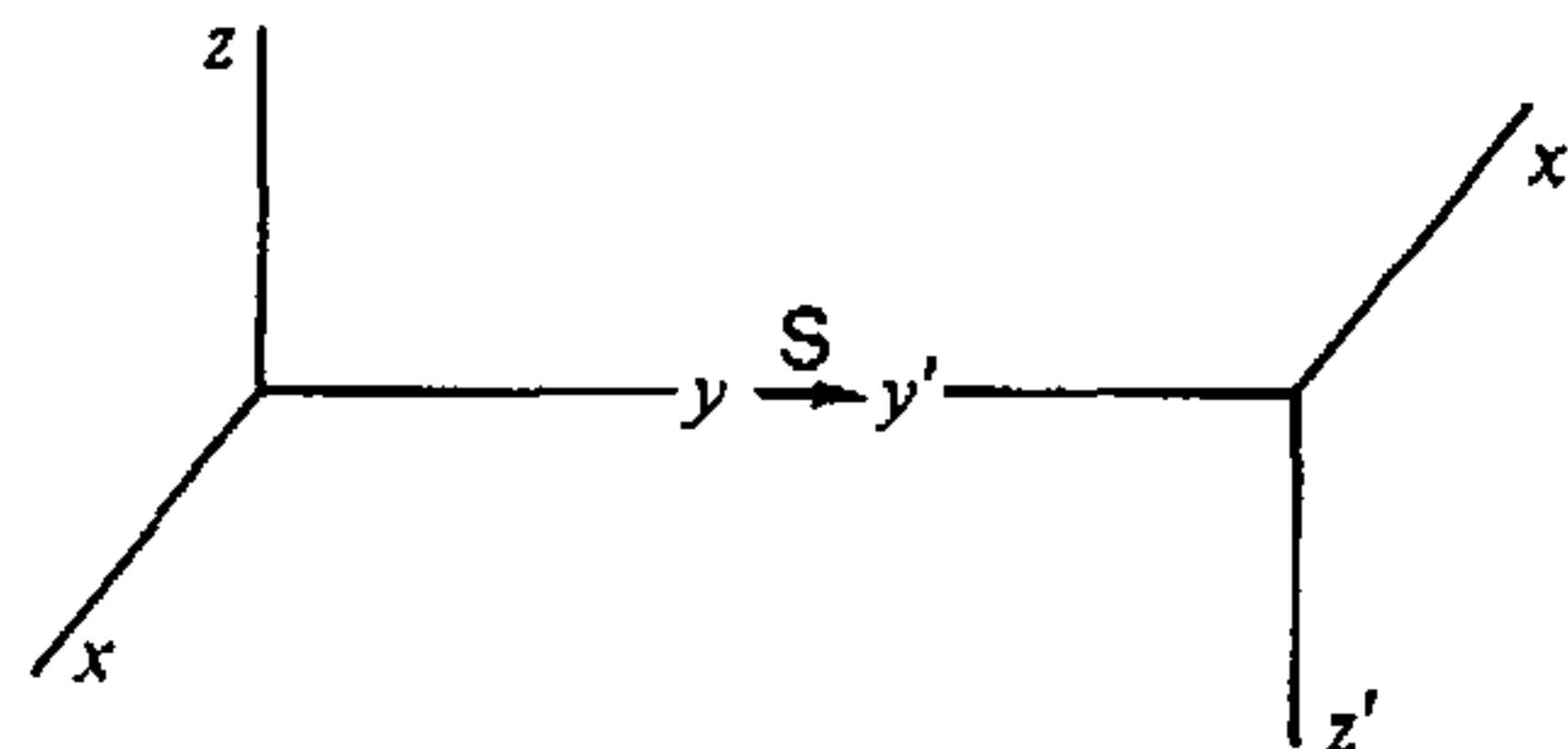
FIGURE 4.6 Inversion of the coordinate axes.
