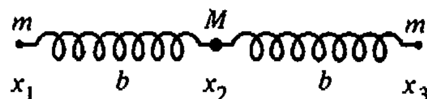
FIGURE 6.3 Model of a linear symmetrical triatomic molecule.
