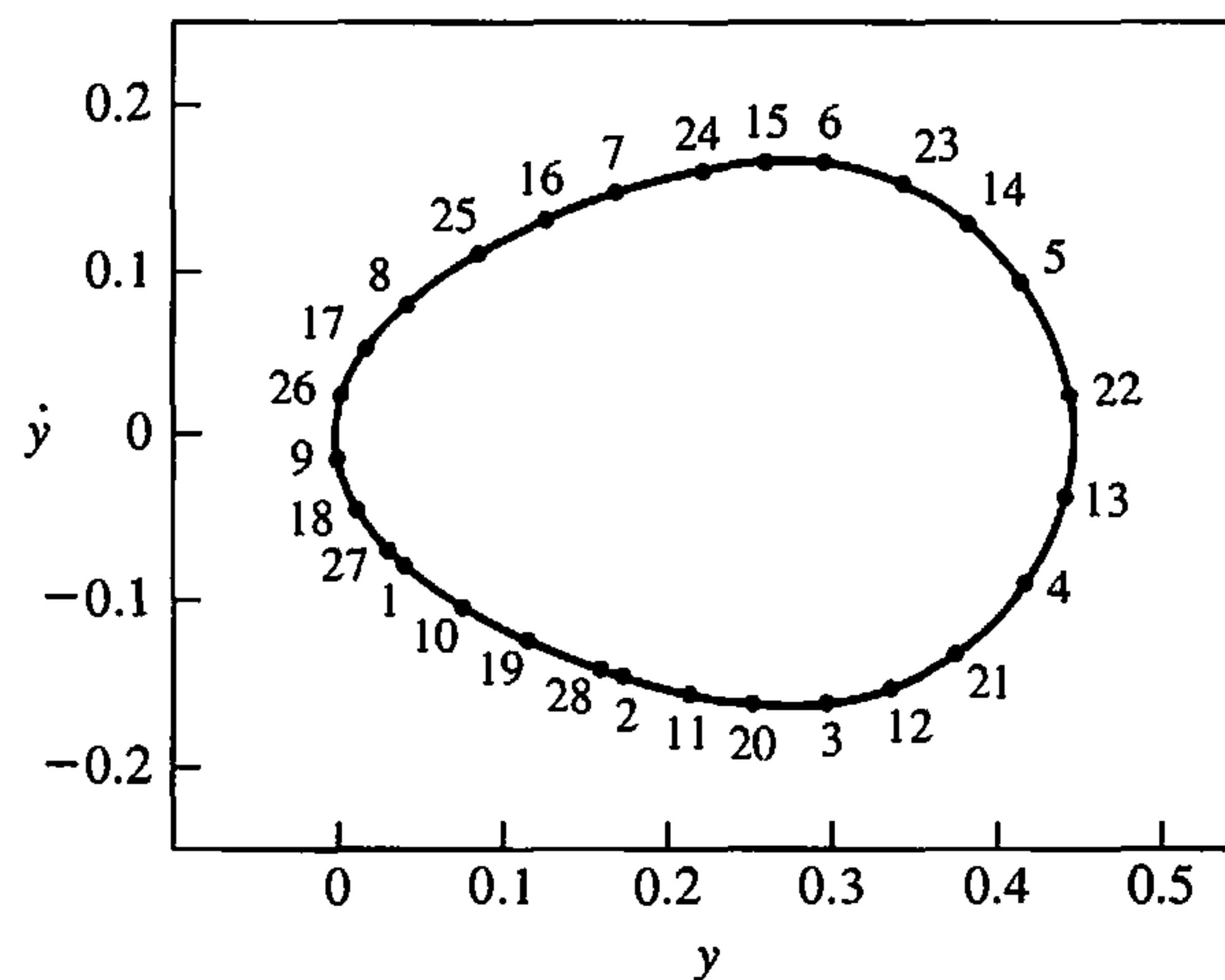
FIGURE 11.7 Poincaré section in the \dot{y}y plane showing the successive points 1, 2, 3, \dots of a Hénon–Heiles orbit for the energy E = \frac{1}{12} . This particular curve also appears on the right side of Fig. 11.8a. From M. Hénon (1983), Fig. 20.
