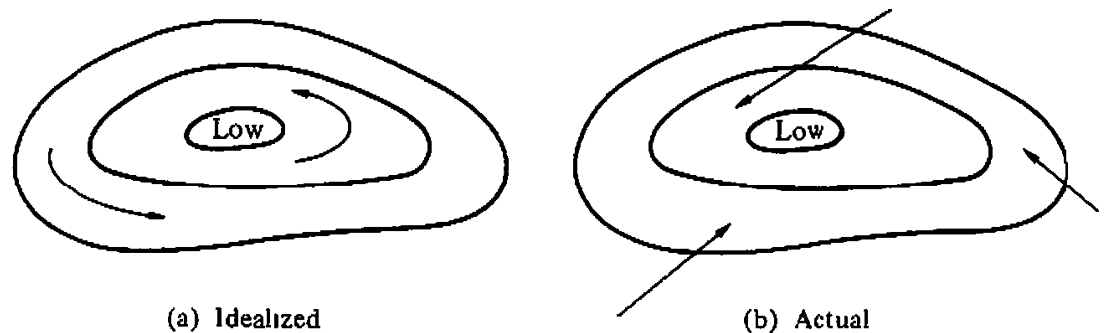
FIGURE 4.15 Cyclone pattern in the northern hemisphere.
