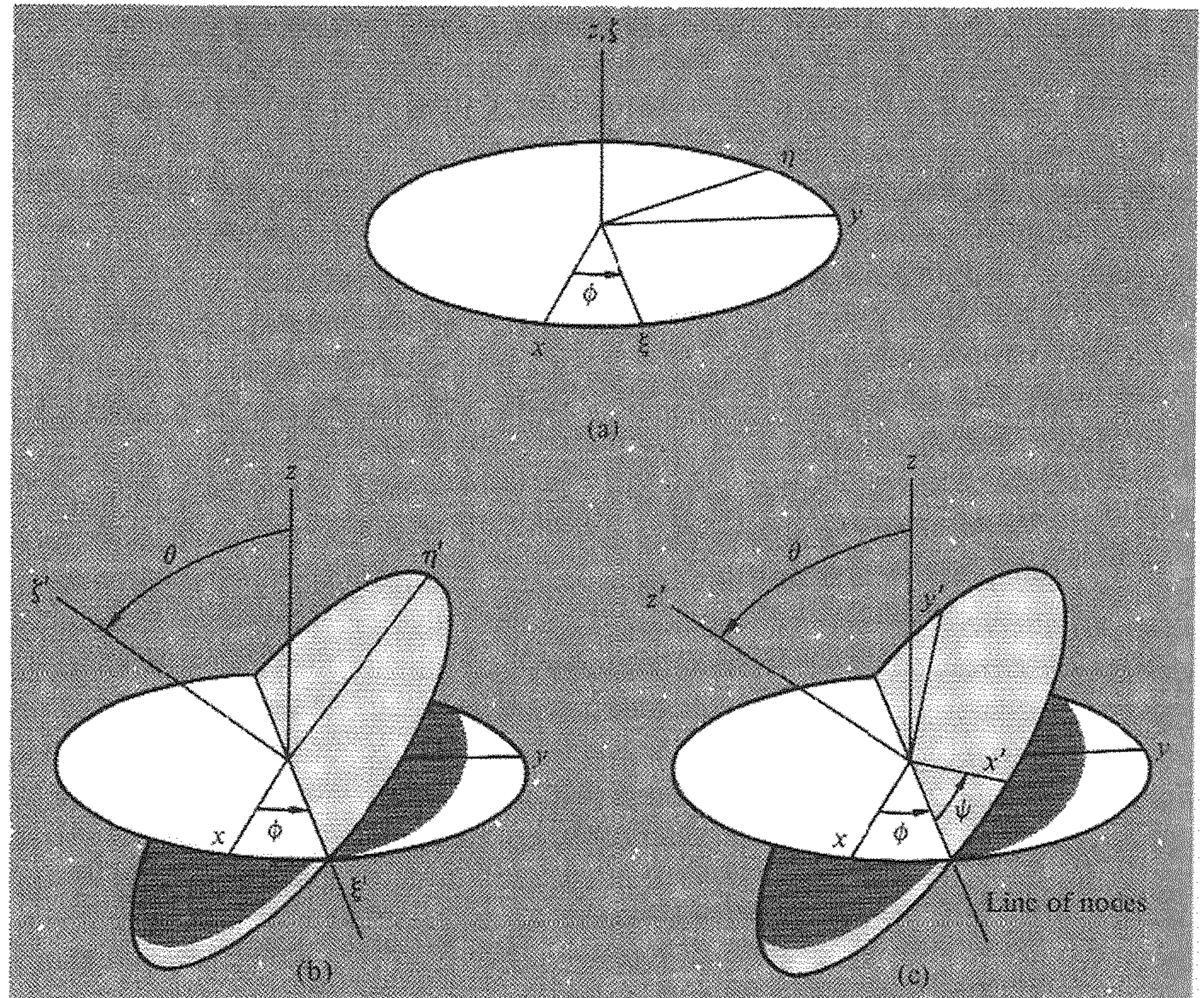
FIGURE 4.7 The rotations defining the Eulerian angles.
