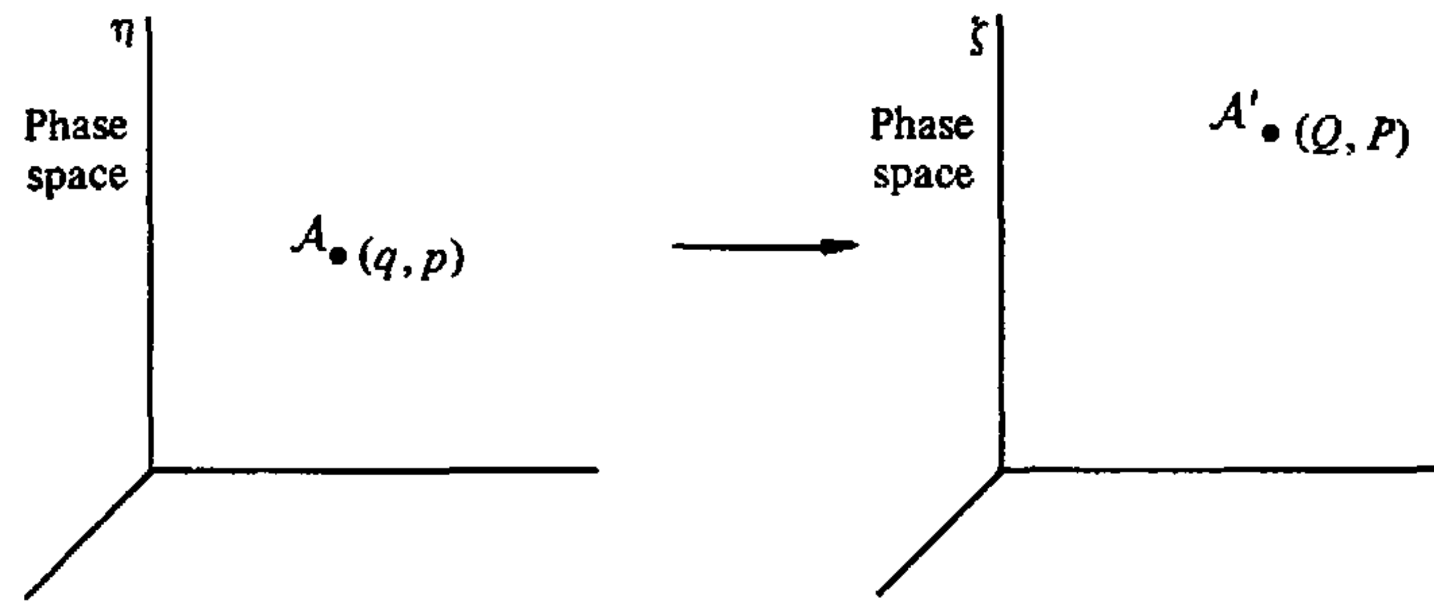
FIGURE 9.2 The passive view of a canonical transformation.
