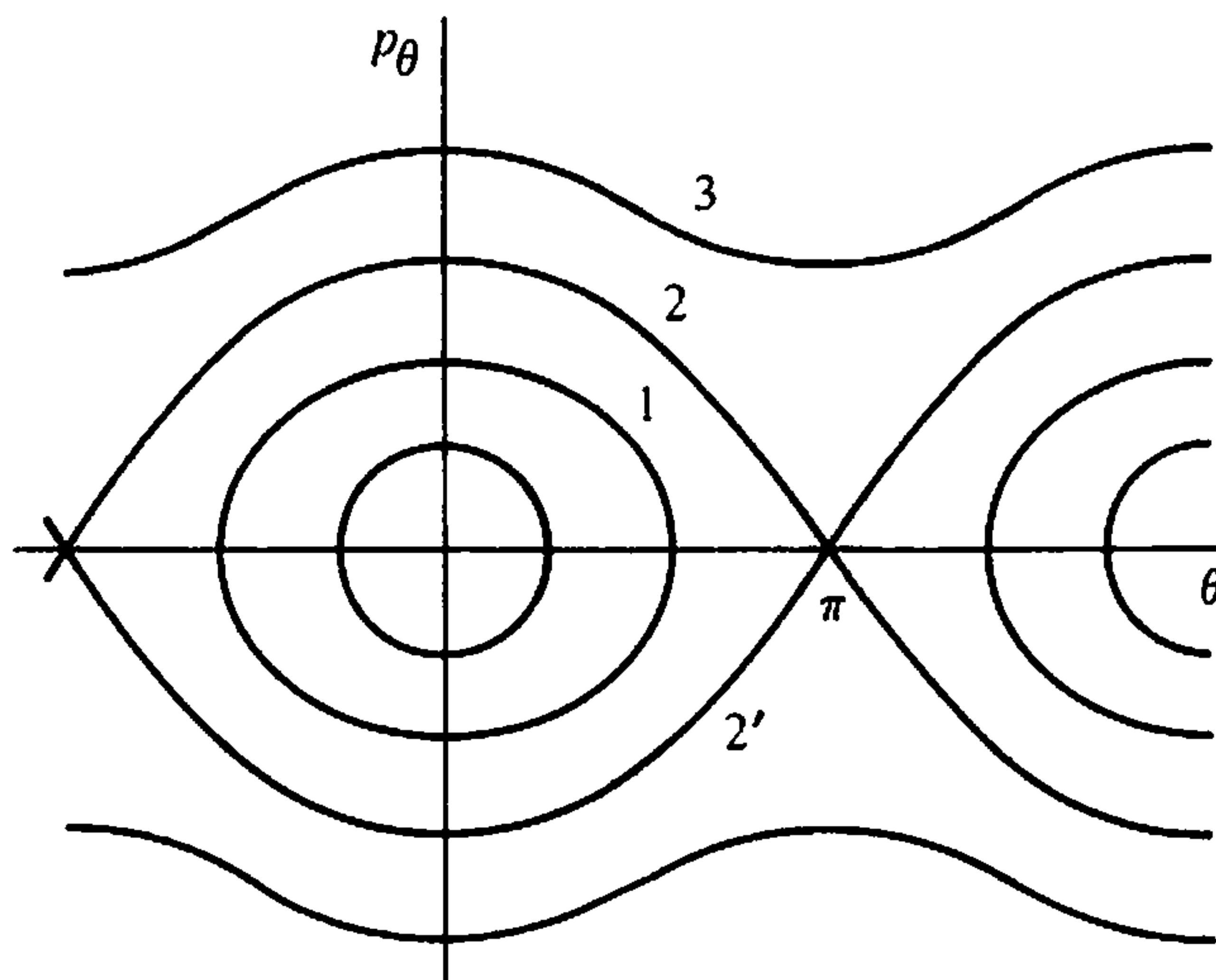
FIGURE 10.3 Phase space orbits for the simple pendulum.
