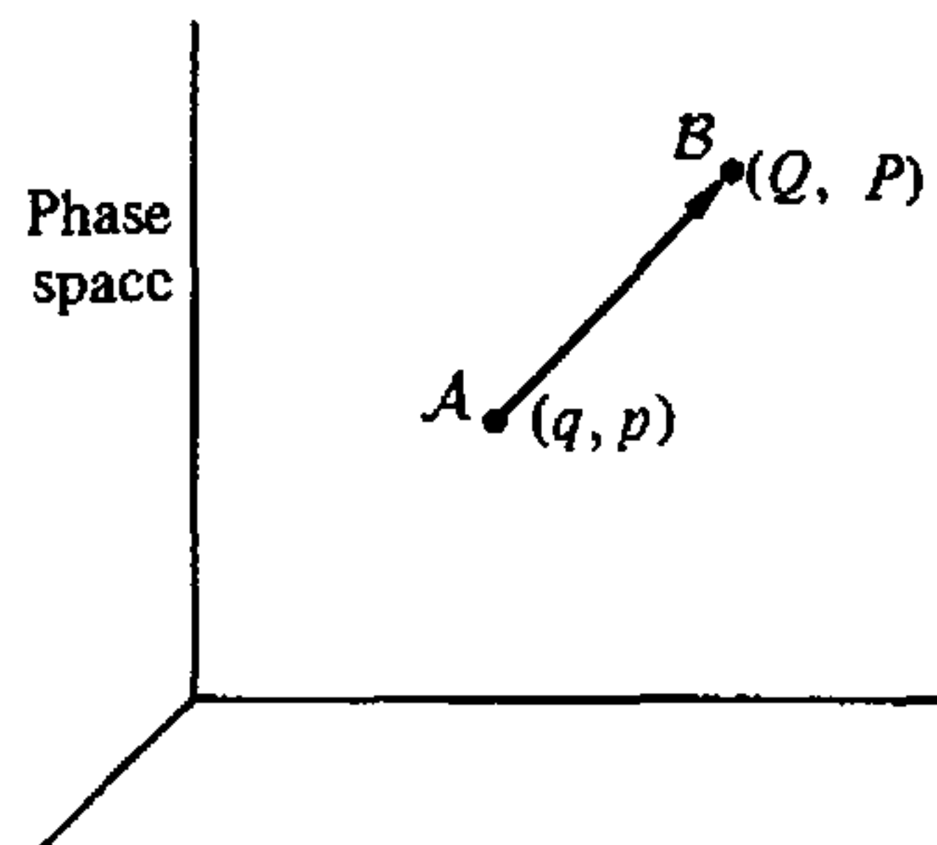
FIGURE 9.3 The active view of a canonical transformation.
