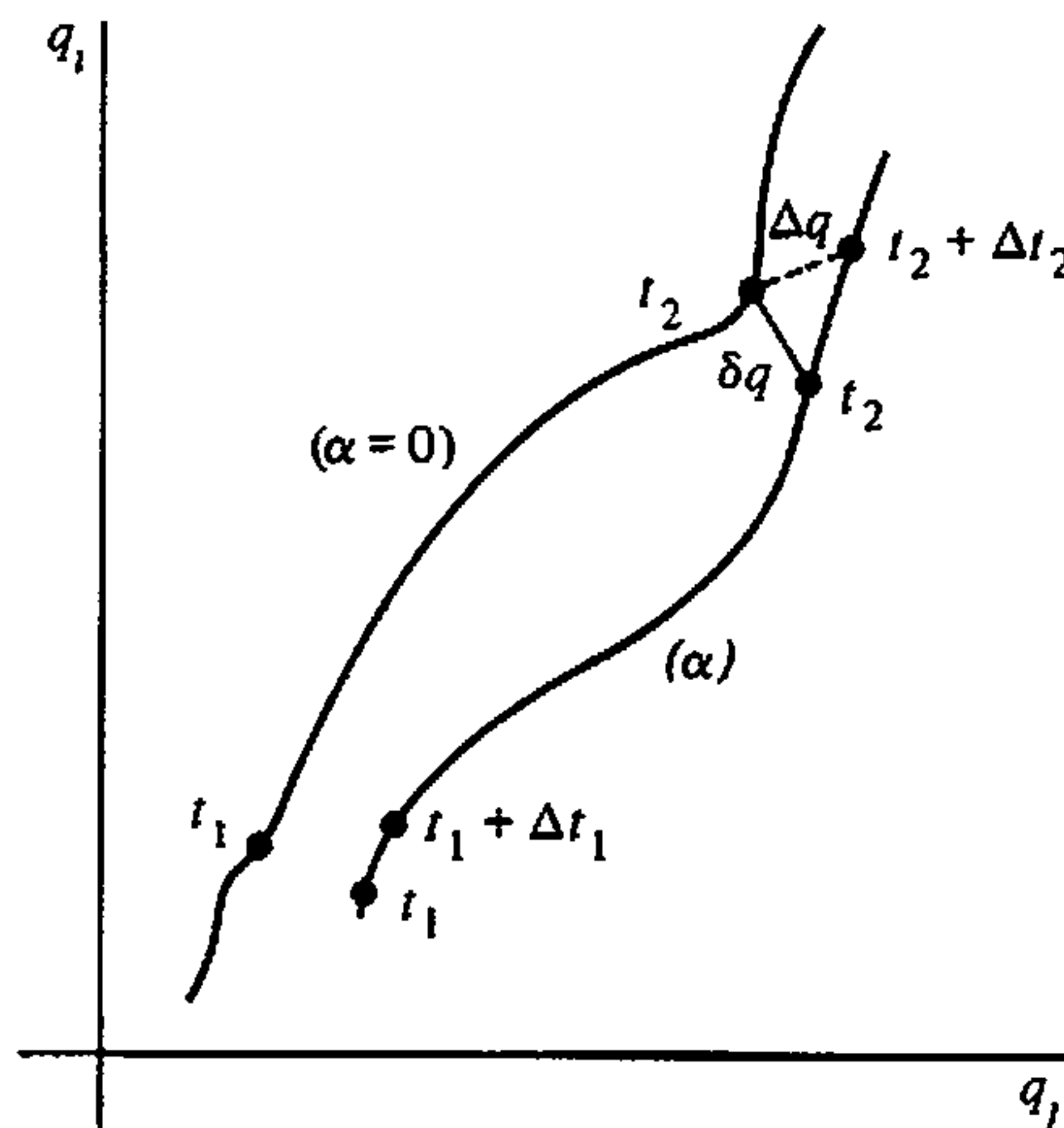
FIGURE 8.3 The \Delta -variation in configuration space.
