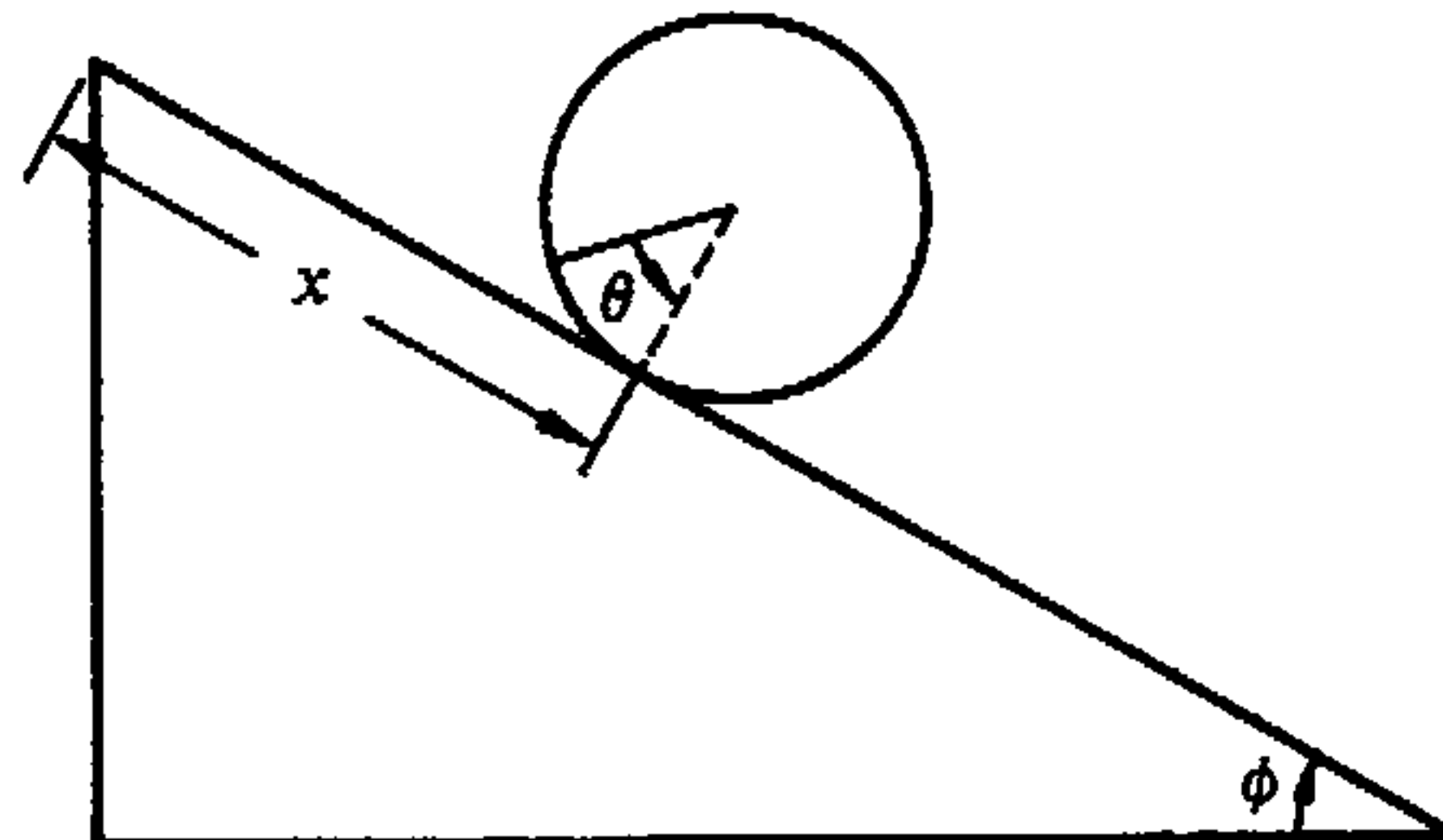
FIGURE 2.5 A hoop rolling down an inclined plane.
