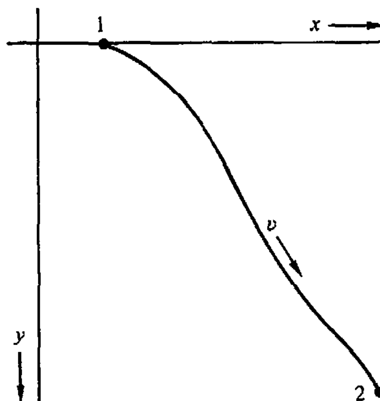
FIGURE 2.4a The brachistochrone problem.
