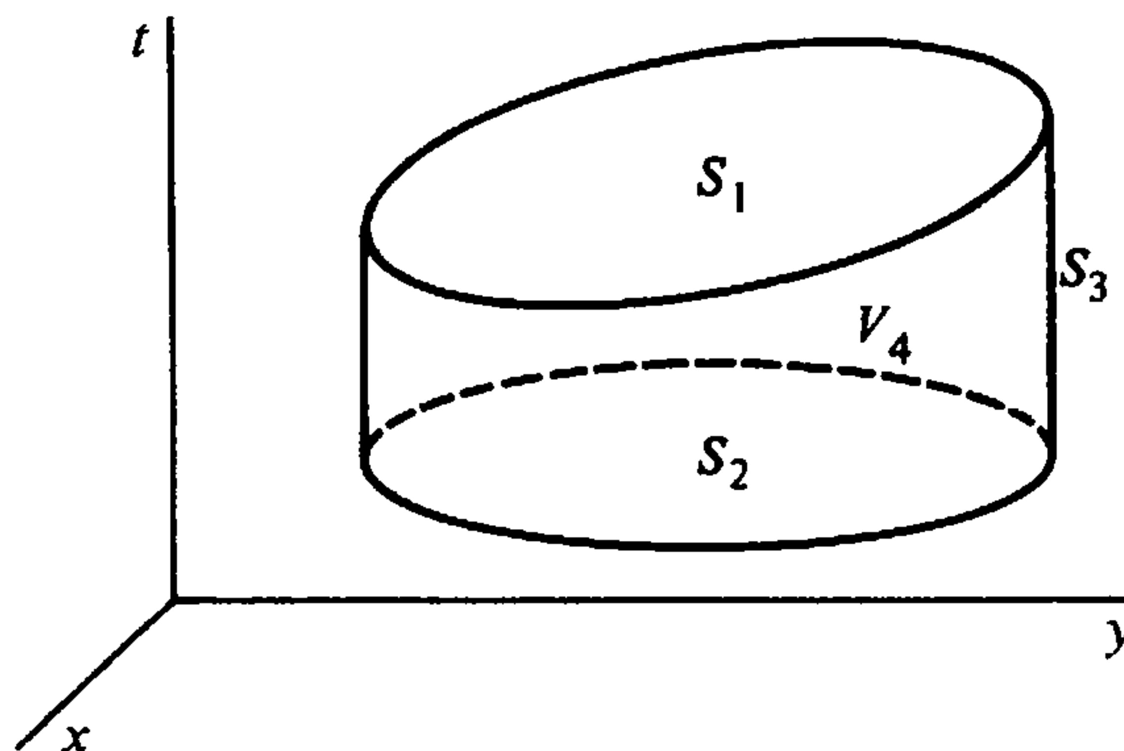
FIGURE 13.5 Schematic integration volume in 4-space
