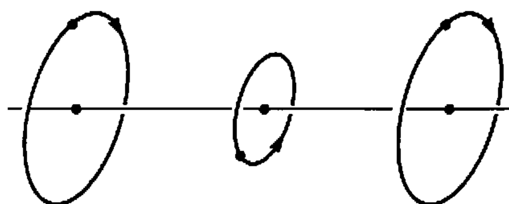
FIGURE 6.5 Degenerate modes of the symmetrical triatomic molecule.
