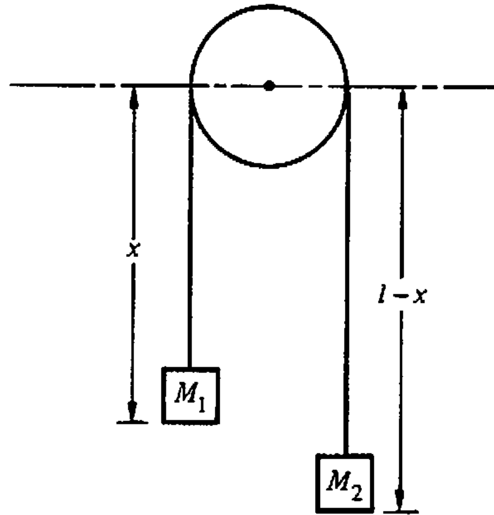
FIGURE 1.7 Atwood's machine.
