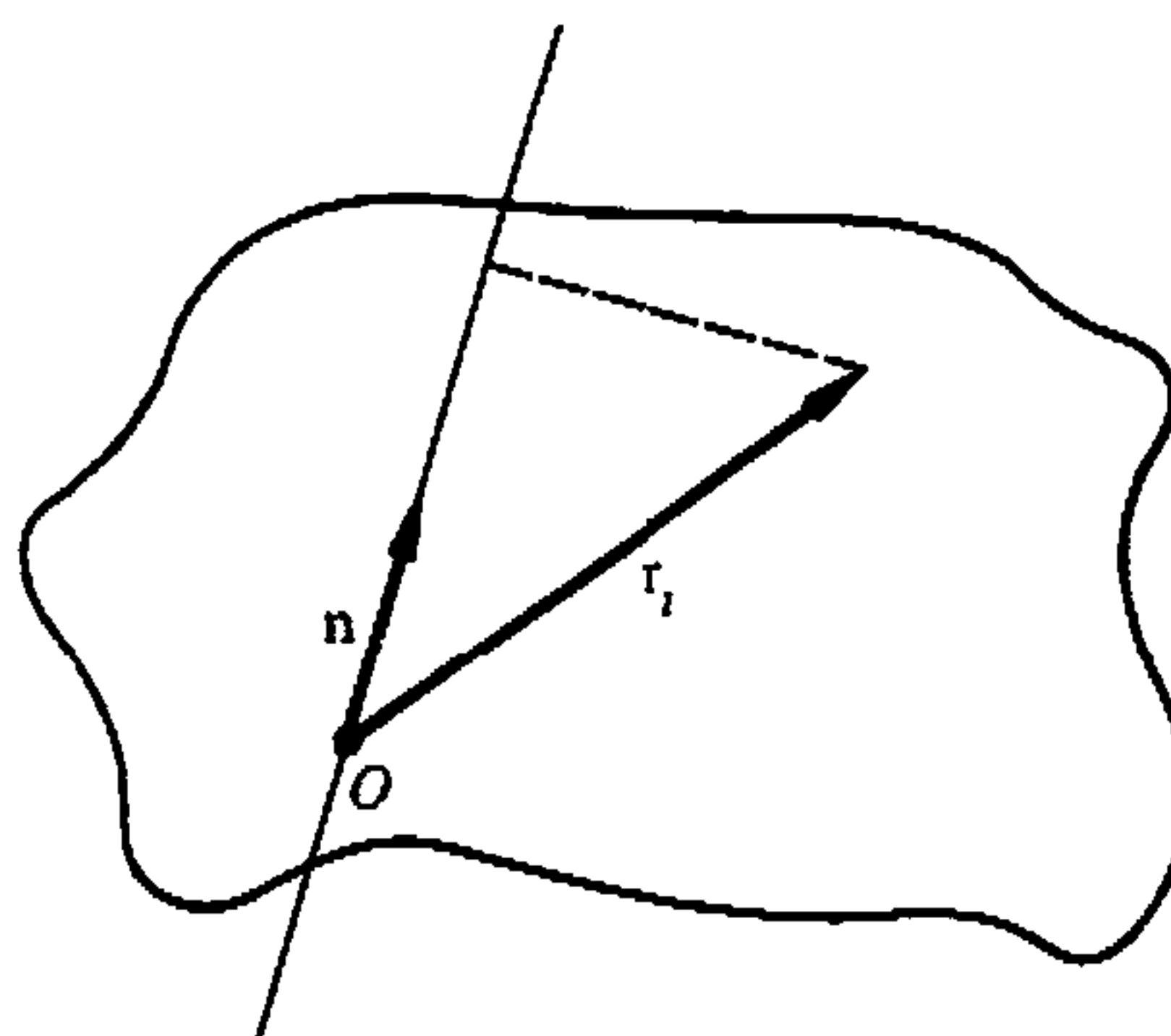
FIGURE 5.2 The definition of the moment of inertia.
