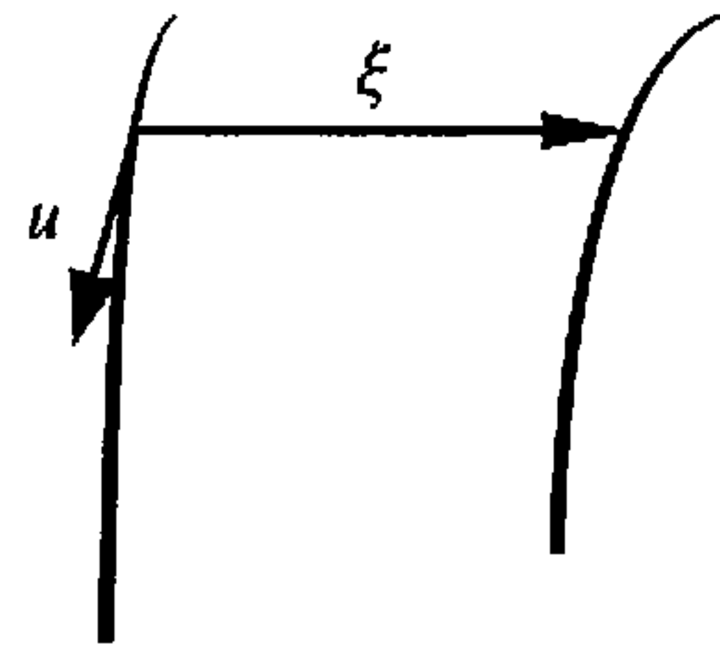
FIGURE 7.5 Tangent vector, u , and deviation vector, \xi .
