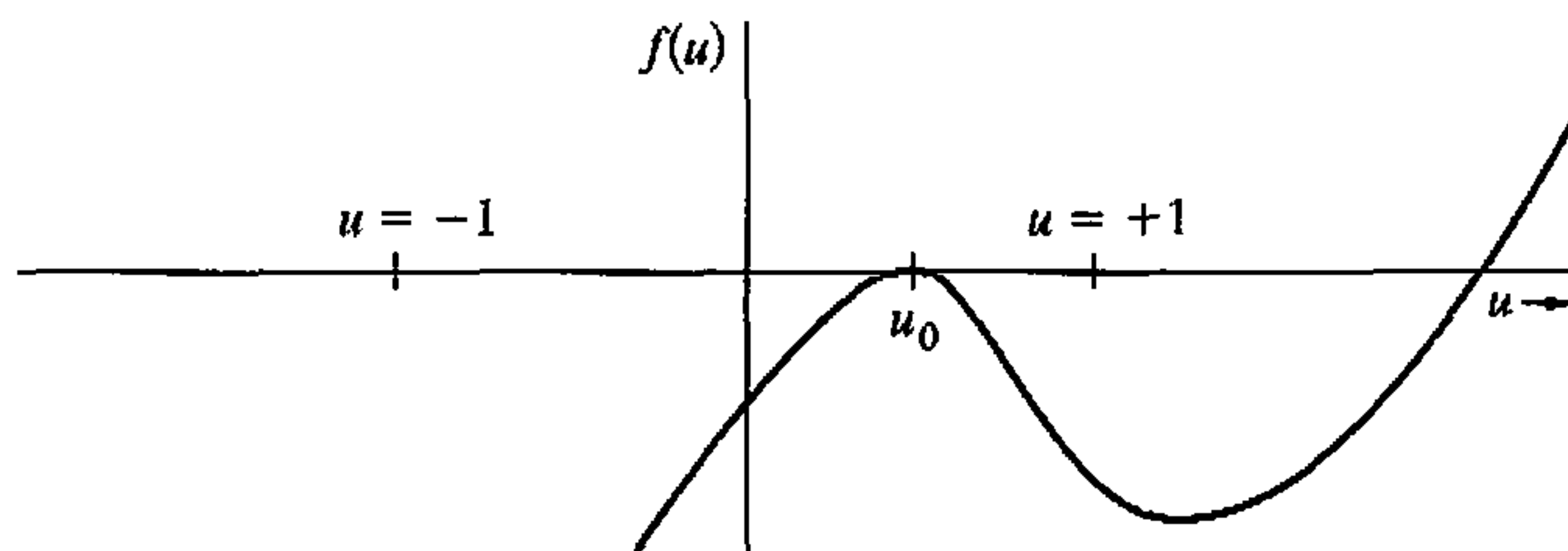
FIGURE 5.10 Appearance of f(u) for a regular precession.
