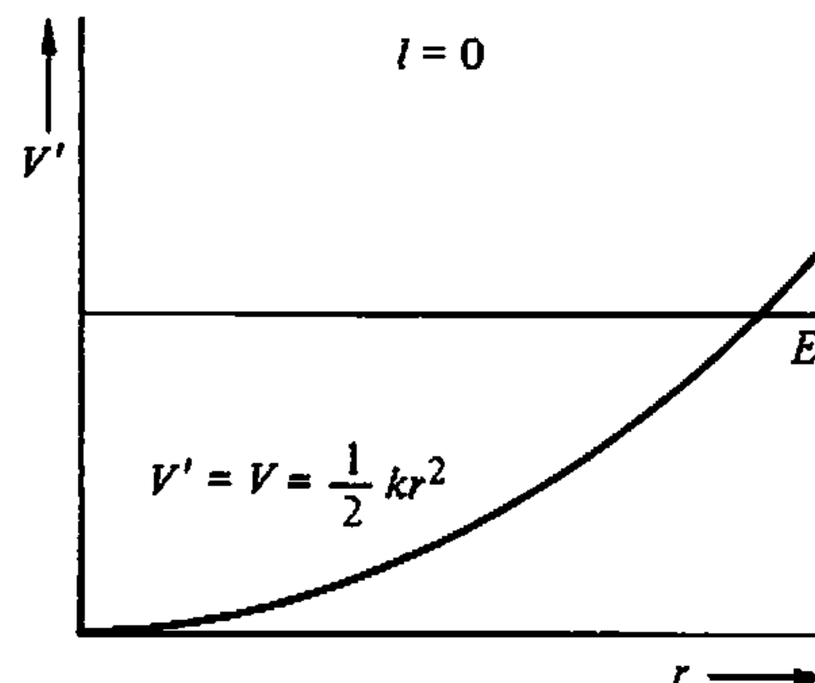
FIGURE 3.10 Effective potential for zero angular momentum.
