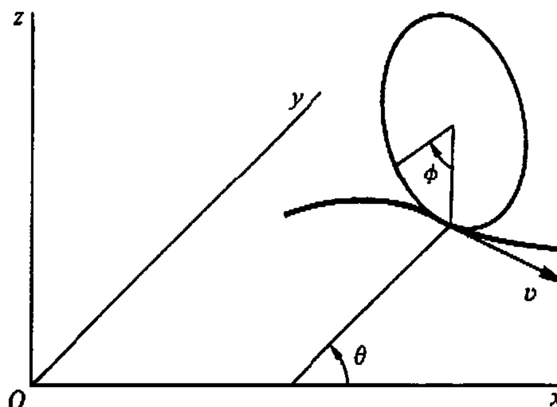
FIGURE 1.5 Vertical disk rolling on a horizontal plane.
