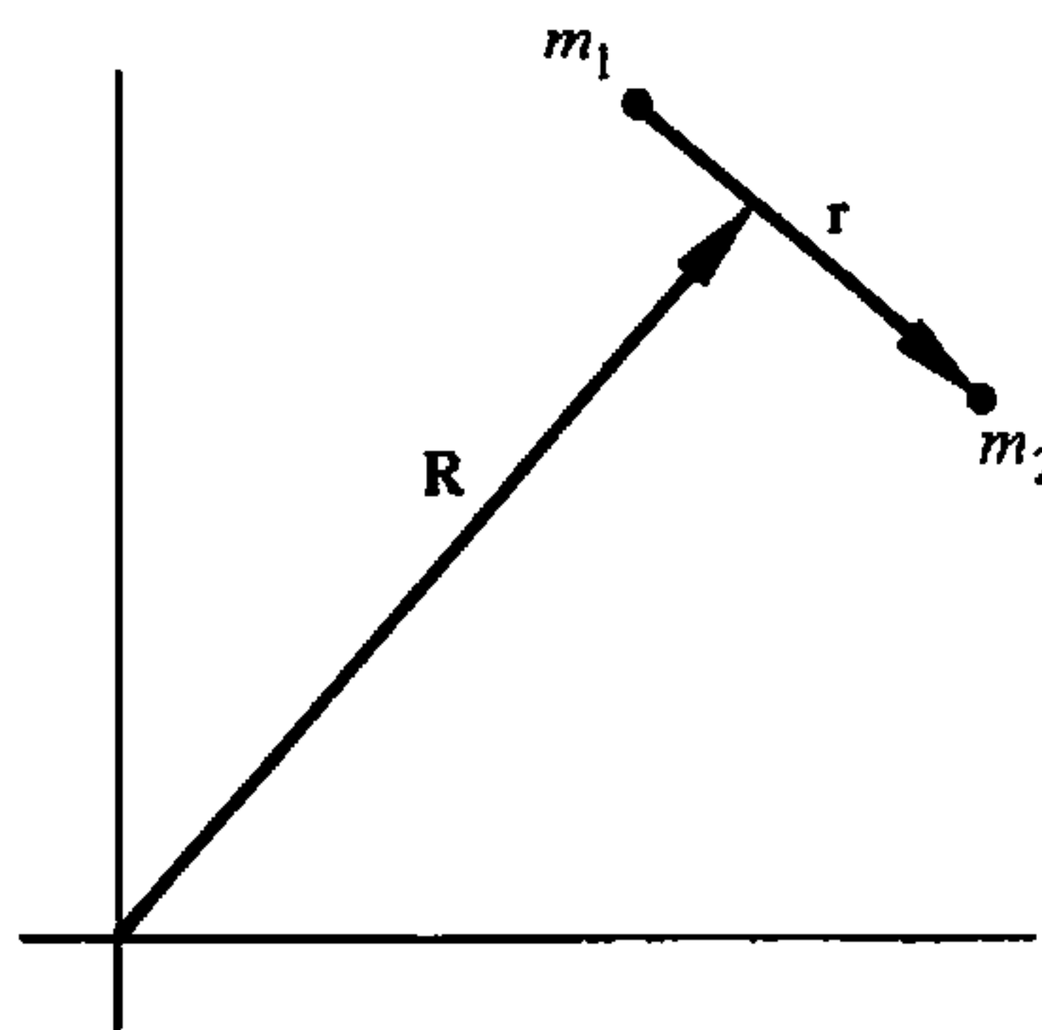
FIGURE 3.1 Coordinates for the two-body problem.
