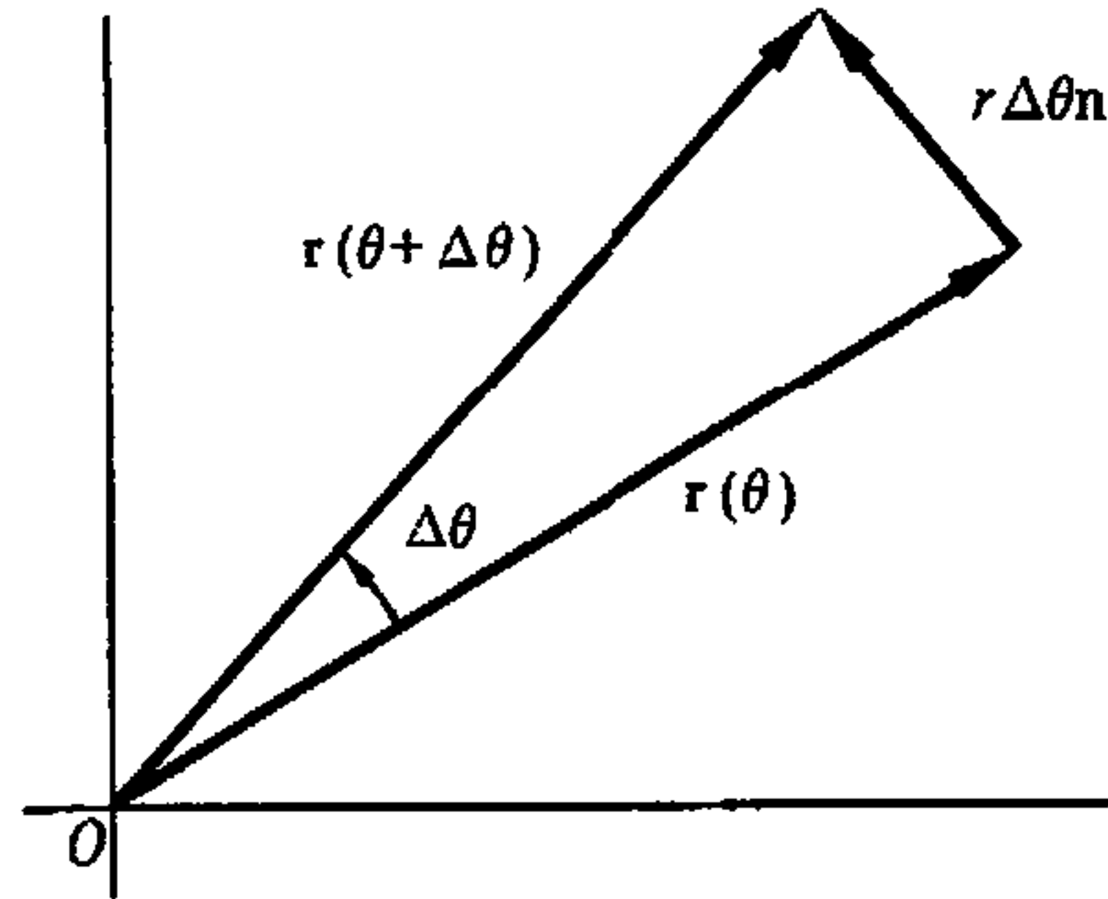
FIGURE 1.6 Derivative of r with respect to \theta .
