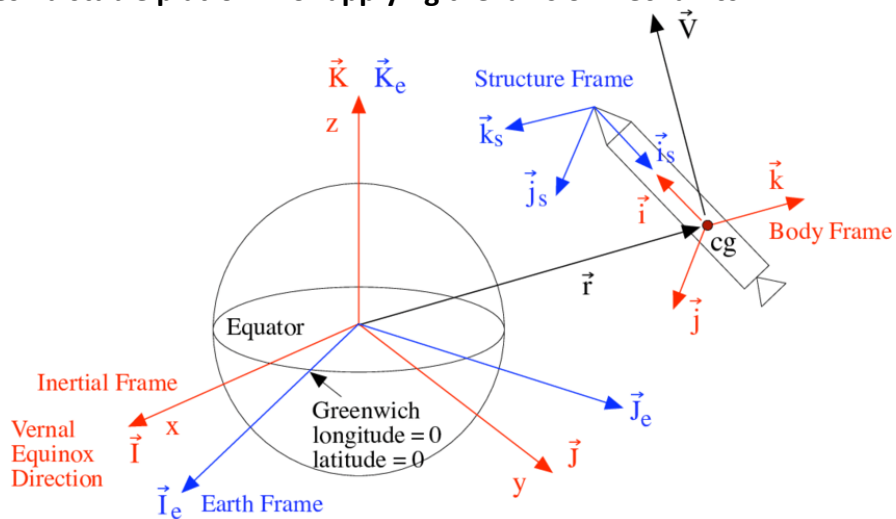
The Earth frame as a reference frame for all motion
