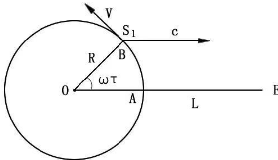
Fig. 5 The schematic picture of calculating charm star.
