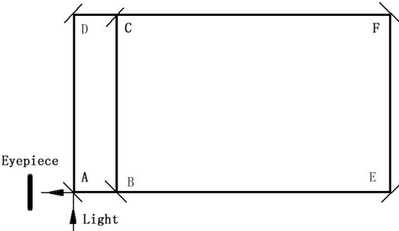
Fig.11 The schematic picture of the M-G experiment.
