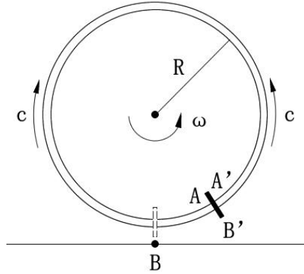
Fig. 9 The calculation diagram of special relativity for the Sagnac effect of hollow fiber loop
