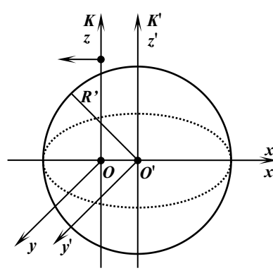
Fig.1 Image 1 of invariable speed of light. Fig.2 Image 2 of invariable speed of light.
