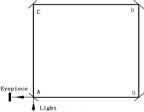
Fig.7 The original experiment diagram of Sagnac effect
