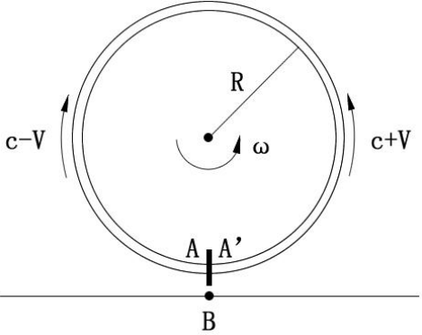
Fig. 8 The calculation diagram of Newton mechanical for the Sagnac effect of hollow fiber loop
