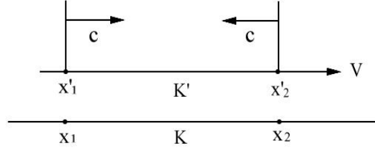
Fig. 6 The time difference of two-way light signals.
