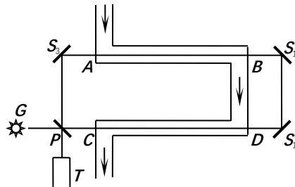
Fig.10 The Fizeau's flowing water experiment
