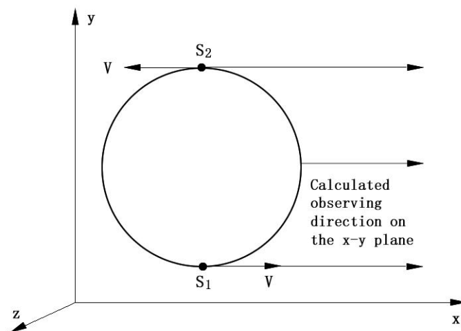
Fig.4 The calculated observing direction and practically observing direction are different resulting in non-observable of orbital shape's change of binary stars.
