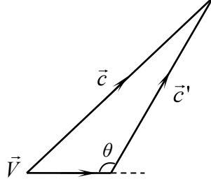
Fig.3 The light's velocities in the cosmic absolute reference frame and the earth's moving reference frame.
