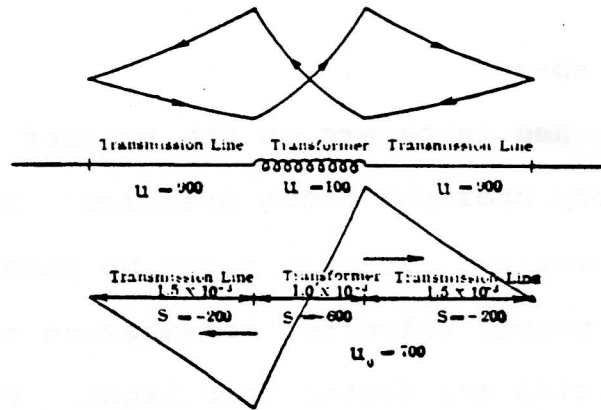
— Energy Distribution in Compound Oscillation of Open Circuit.
