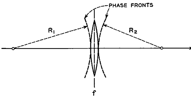
Fig. 1 — Lens transforming phase front of spherical wave.
