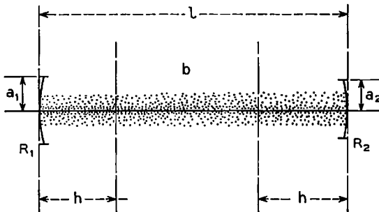
Fig. 15 — Resonator with an internal lenslike medium.
