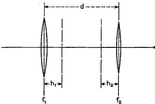
Fig. 5 — The two-lens combination.
