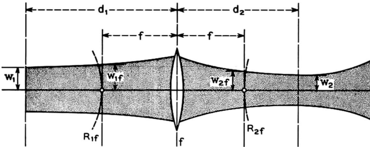
Fig. 10 — Gaussian beam transformed by a lens.
