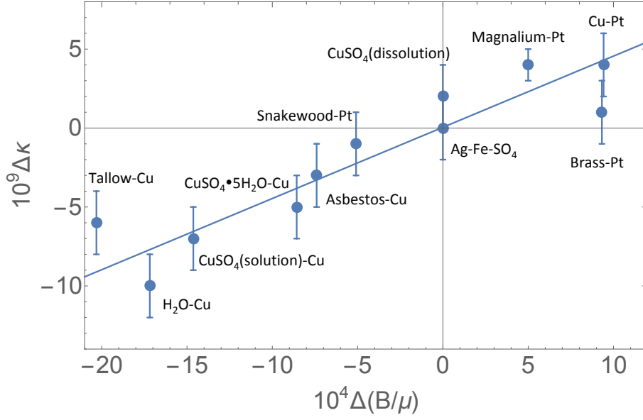
Figure 1: Plot of the data from Table 1 with the best fit line from Ref. [8], revealing a dependence of \kappa on the baryon-to-mass ratio.
