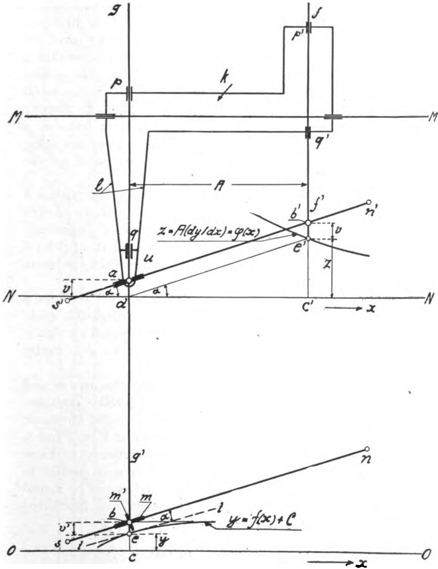
FIG. 1. The principle of the Integraph.
