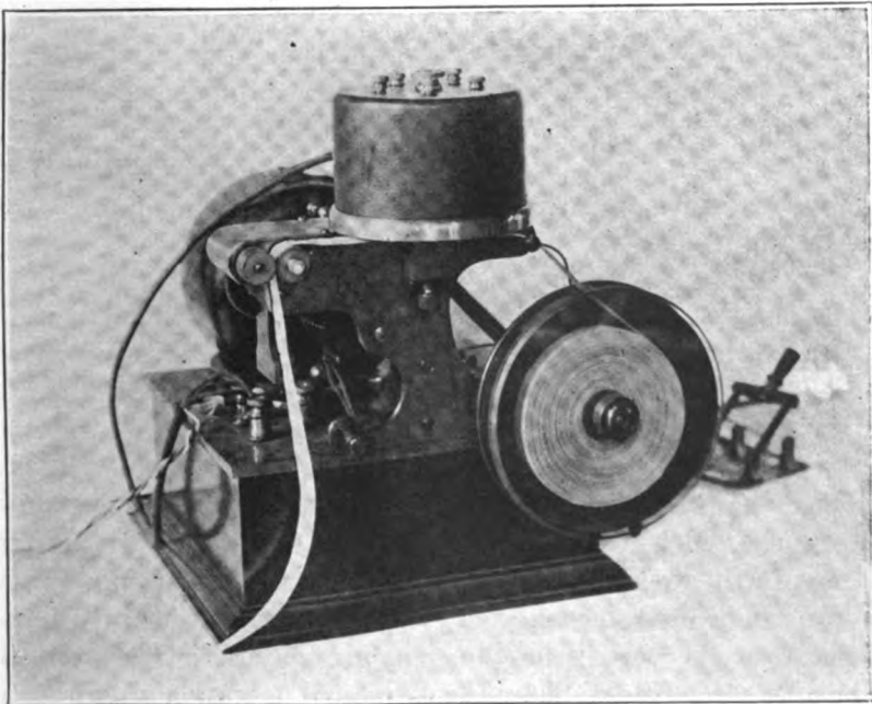
FIG. 5—Receiver
