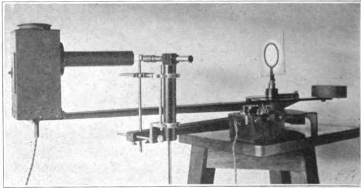
FIG. 2—Photograph of Apparatus
