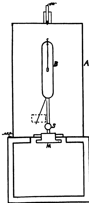
FIG. 1. Bothe's electroscope
