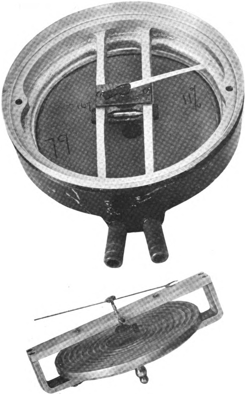
FIG. (C). Ogilvie rubber diaphragm (above) Sperry single diaphragm (lower) Air Speed Indicators
