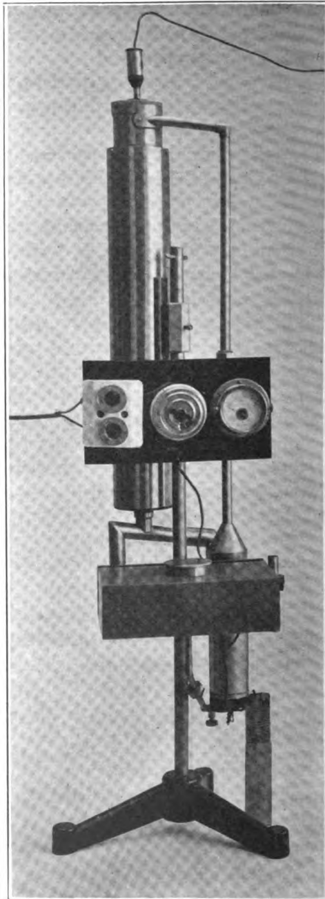
FIG. 1. Laboratory Hypsometer
