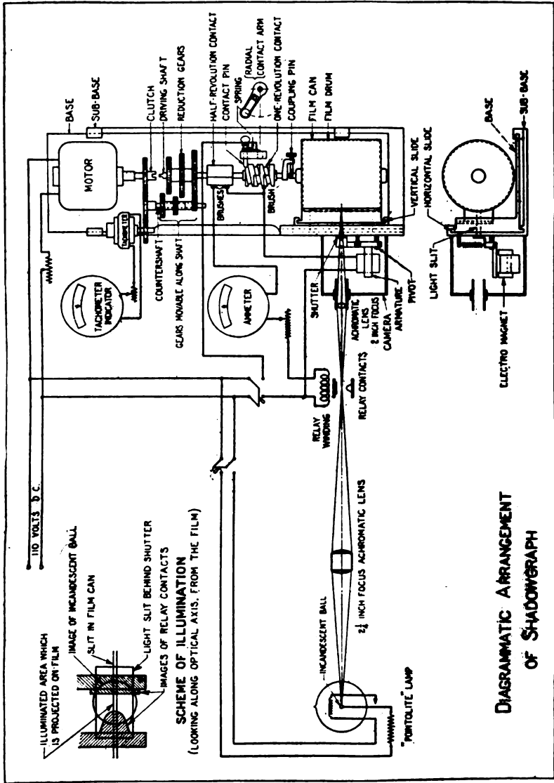
FIG. 1 Diagrammatic sketch of shadowgraph and connections.
