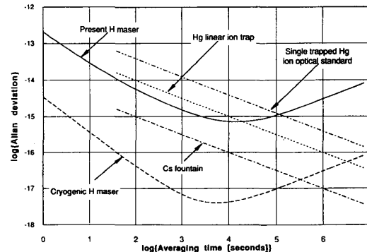
Fig. 1. Predicted Allan variance for future frequency standards [1]. (This assumes no systematic effects in Cs and Hg devices.)
