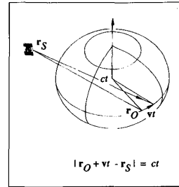
Fig. 7. Propagation of a signal from a satellite at position r_S to a receiver which moves a distance vt during the propagation time. The Sagnac effect will be automatically included if receiver motion due to earth rotation during signal propagation is accounted for.
