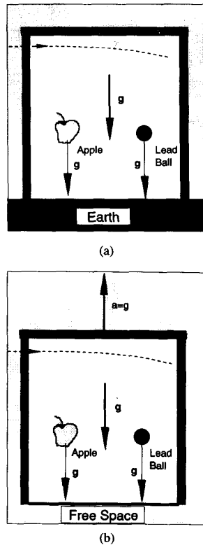
Fig. 9. (a) Laboratory near the earth's surface where the acceleration due to gravity is g . All objects fall with equal accelerations. (b) By the Equivalence Principle, experiments performed in an accelerated lab in free space have the same outcomes.
