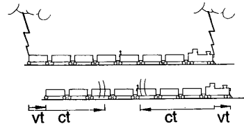
Fig. 4. Thought experiment illustrating relativity of simultaneity.
