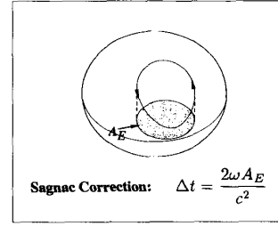
Fig. 5. For a sequence of Einstein synchronization processes around the closed circuit on the rotating earth's surface, the Sagnac effect is proportional to the shaded area, which is the area enclosed by the circuit, projected onto the earth's equatorial plane.
