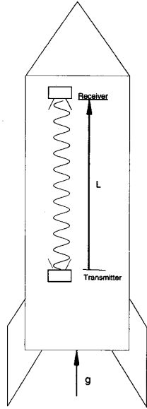
Fig. 10. A signal traveling upwards in a gravitational field is shifted towards lower frequencies.
