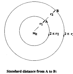
Fig. 12. Effect of spatial curvature on standard distance measurements.
