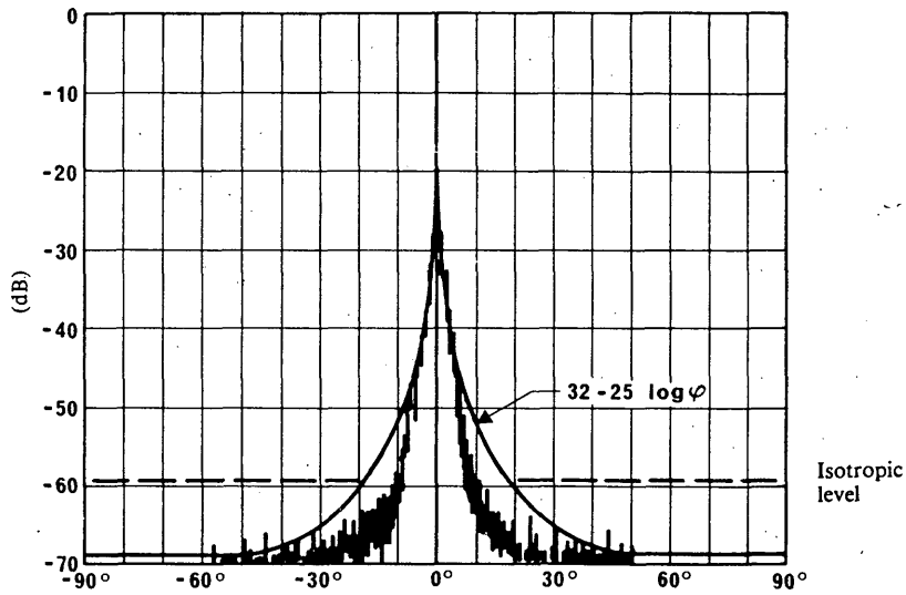
b) Curved struts with special scattering surface
