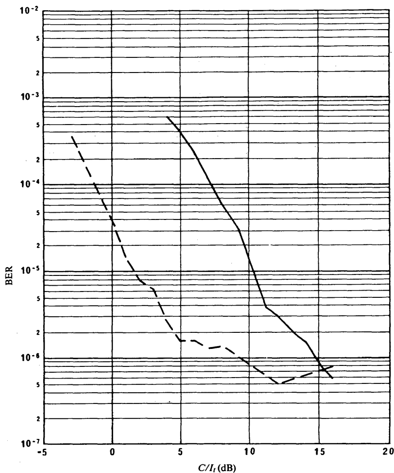
FIGURE 5c - BER as a function of the level of the TV carrier ( I_1 ) modulated by a colour bar picture in the PAL system for two different frequency dispersal wave forms
