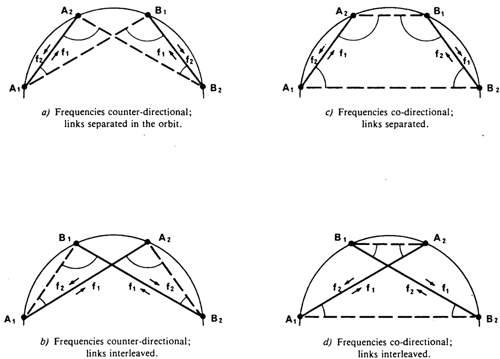
FIGURE 3 — Interference geometries between inter-satellite links (Angles marked are antenna discrimination angles. Interference paths are shown in broken lines.)
