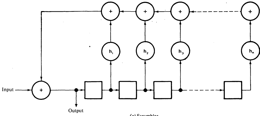
(a) Scrambler
