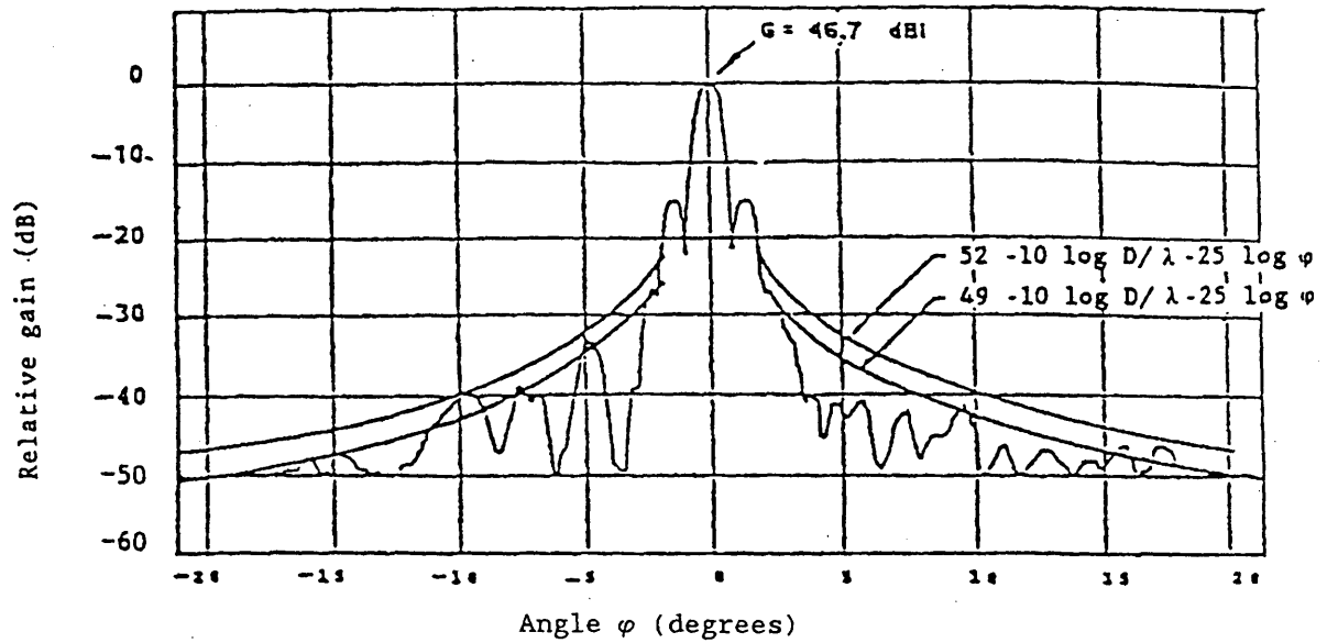
FIGURE 6 - Measured radiation pattern of a 4.5 m Cassegrain antenna in the azimuth plane
