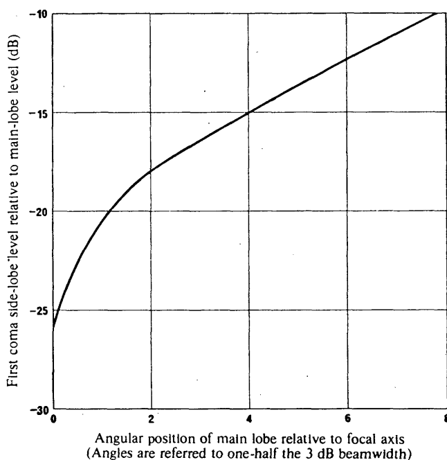
FIGURE 5 – First coma side-lobe level versus angular position of main lobe relative to focal axis
