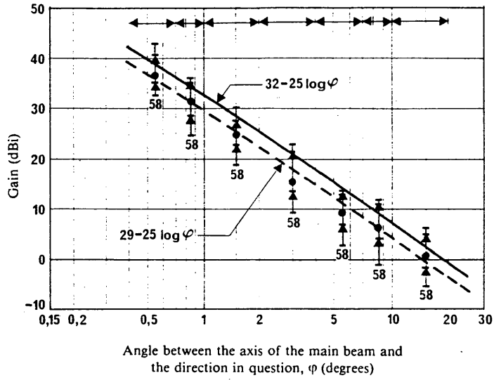
FIGURE 2a - Distribution of side-lobe levels in circularly polarized co-polar patterns for INTELSAT Standard A Antennas
