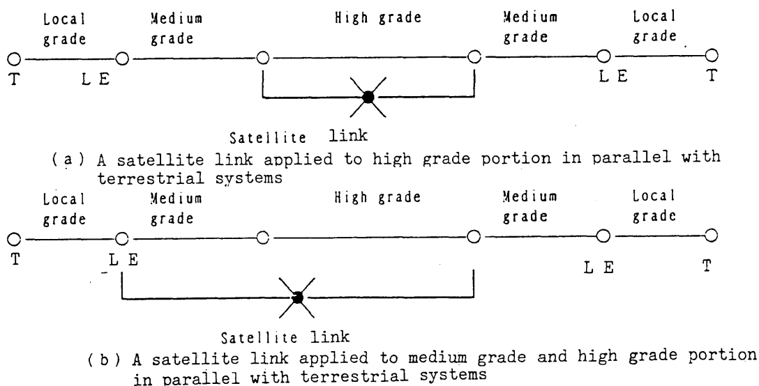
FIGURE 3 - Configuration examples of satellite links applied to one or several sections of the digital path in parallel with terrestrial systems
