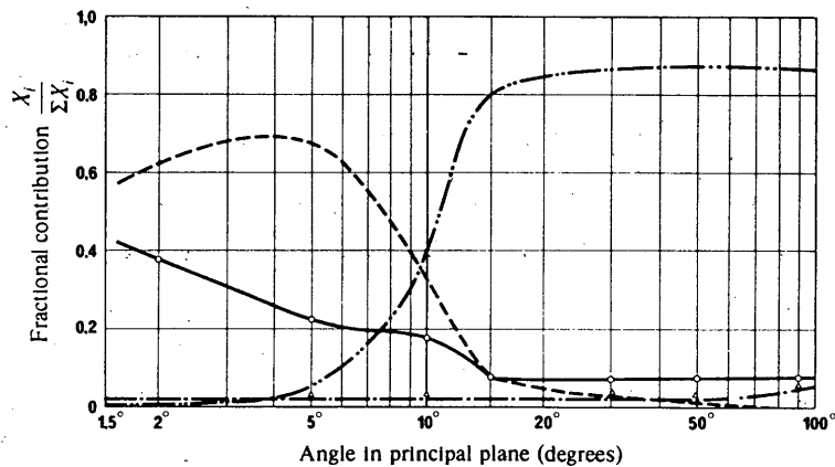
FIGURE 1 — Relative contribution of various parts of 600 λ Cassegrain antenna to wide angle gain envelope
