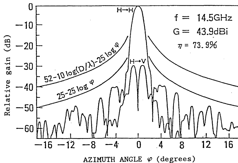
FIGURE 13 - Measured radiation patterns of 1.2 m shaped offset Gregorian antenna ( f = 14.5 GHz, D/\lambda = 58 )
