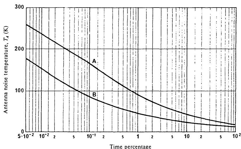
FIGURE 1 - Measured antenna temperature as a function of the percentage of time each level was exceeded
