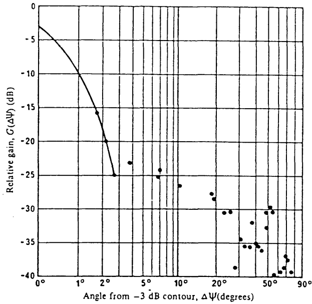
FIGURE 27 - Out-of-beam data for 61 element feed array satellite lens antenna Frequency = 8 GHz -3 dB beamwidth = 20°
