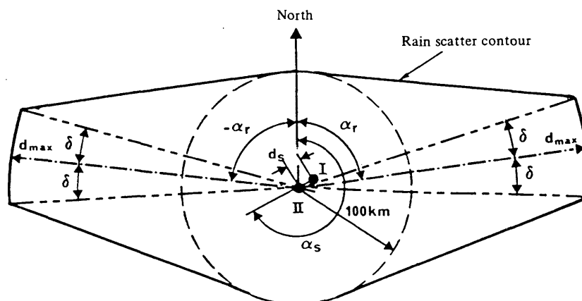
FIGURE 7 – Example of bidirectional rain scatter area
