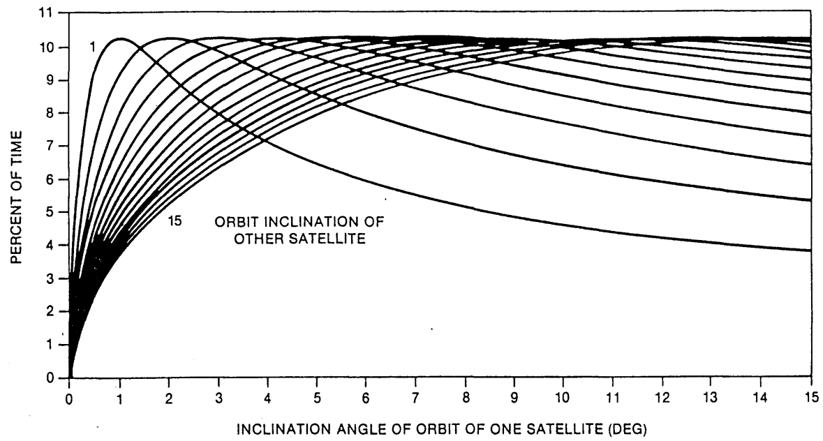
FIGURE 5. Percent of Time Satellite Spacing is Less Than Nodal Spacing
