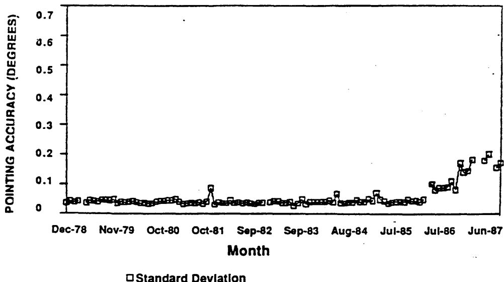
Figure 3 - IVA-F6 pointing performance. Launch to end-of-life
