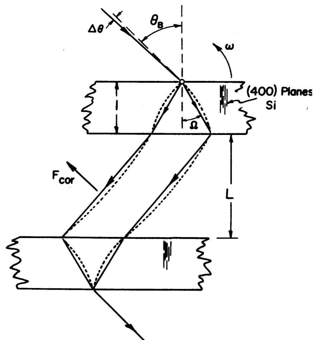
FIG. 1. Typical neutron current flow in a two-crystal interferometer without rotational motion of interferometer (solid lines) and with rotational motion about entrance point (dashed lines). Overlap focusing occurs at an exit point for either case (slightly modified entrance conditions are necessary to maintain the same separation of the illustrated beams) when a suitable wedge is positioned in the gap between the crystals. The trajectory curvature, arising from the Coriolis force on the neutrons, is very much larger (and with both signs) within the crystals than in the free space region.
