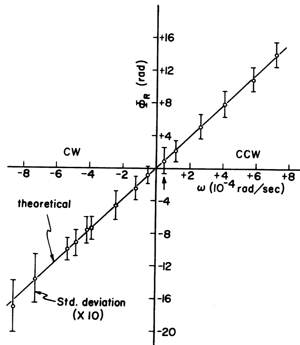
FIG. 3. Interferometer phase difference induced by rotation as a function of rotational angular speed. For clarity, the standard-deviation brackets of the measured points are presented with tenfold amplification. The small arrow indicates the effective terrestrial rotation speed at Cambridge, Massachusetts and the solid line is the expected linear dependence of Eq. (6).
