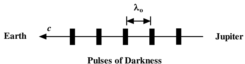
Figure 2. Pulses of darkness from Jupiter-Io system to earth.
