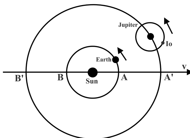
Figure 1. Motion of Sun-Earth-Jupiter system through the ether.
