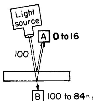
FIGURE 4. An experiment to measure the partial reflection of light by two surfaces of glass. Photons can get to the photomultiplier at A by reflecting off either the front surface or the back surface of the sheet of glass; alternatively, they could go through both surfaces and end up hitting the photomultiplier at B. Depending on the thickness of the glass, 0 to 16 photons out of every 100 get to the photomultiplier at A. These results pose difficulties for any reasonable theory, including the one in Figure 3. It appears that partial reflection can be “turned off” or “amplified” by the presence of an additional surface.
