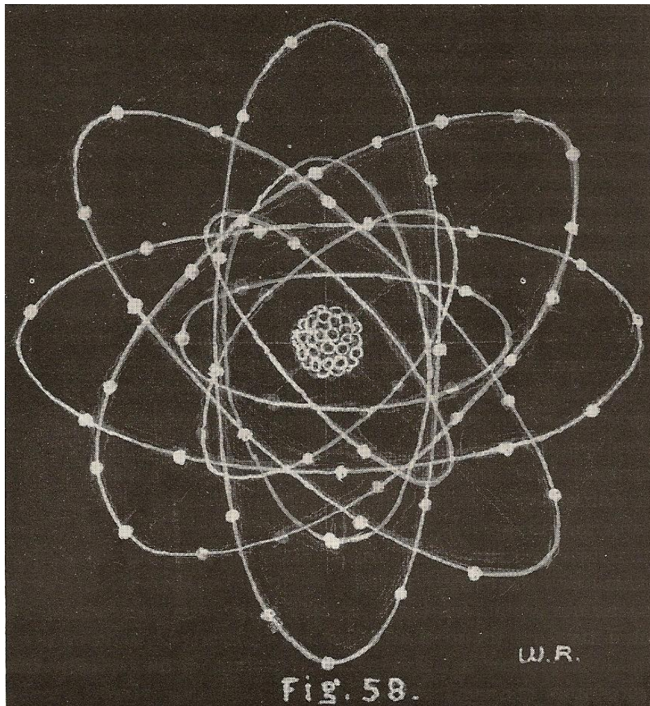
The Rutherford-Bohr atom.
