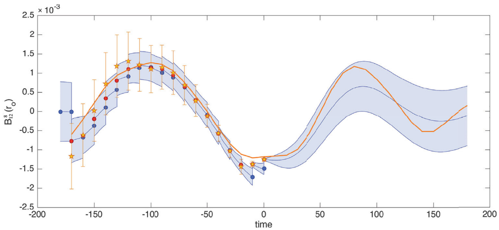
Figure 13. Example of an EnKF data assimilation for the surface magnetic field of degree l = 12 and order m = 8 in a dynamo model. The ensemble mean is given by circles and the error bars show the \sigma confidence interval based on the ensemble spread. After the initialisation, the ensemble assimilates noisy observations (stars) over a sequence of forecast (blue) and analysis (red) cycles and quickly approaches the reference true state from which the observations were created. Though the data assimilation is stopped at t = 0 , the model continues to evolve close to the reference trajectory. For longer time scales, the predictive power naturally degenerates due to the chaotic nature of the system. (Colour online)
