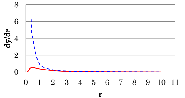
Fig. 13 Plot of equations: the solid line corresponds to \frac{dy}{dr} = \frac{1}{r^2}e^{-\frac{1}{r}} and the dotted line corresponds to \frac{dy}{dr} = \frac{1}{r^2} .
