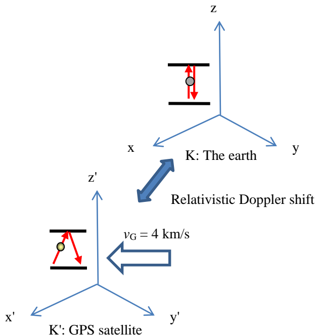
Fig. 2 Counterexample of the principle of relativity
