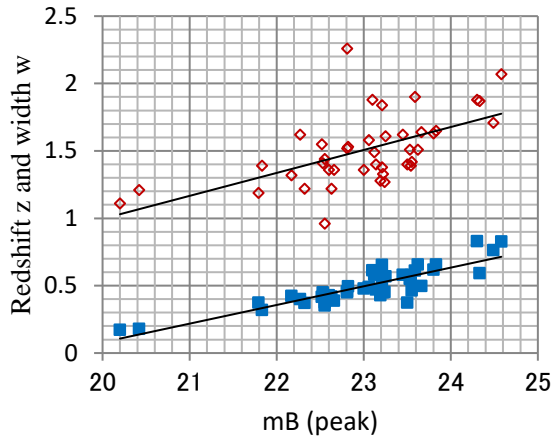
Fig. 24 Magnitude-redshift and light curve width relation of type Ia supernovae (magnitude 20 to 25) using the experimental data by Perlmutter 53 et al. and Goldhaber 54 et al.
