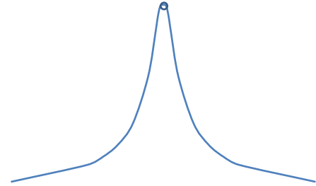
Fig.19 Ether density distribution from point mass simultaneously moves with the point mass. At the same time, the fluctuation travels at the speed of light c , as gravitational waves.
