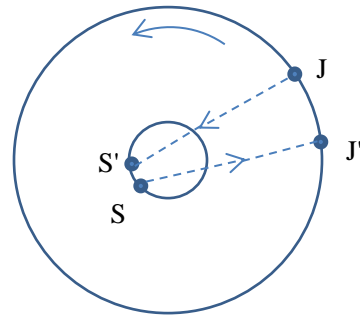
Fig. 21 Copy from Eddington's 36 book (P. 84, FIG. 13)
