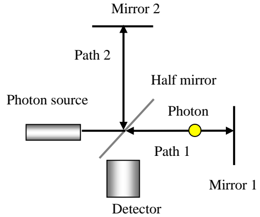
Fig. 5 Single-photon Michelson-Morley experiment 27
