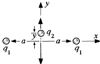
Fig. 10.7 A point charge q_2 oscillates along the y axis under the action of two fixed point charges q_1 . This system can be used as a primitive clock.
