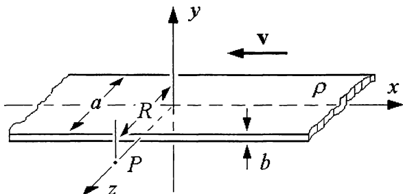
Fig. 5.2 An infinitely long thin ribbon of charge density \rho moves with uniform velocity \mathbf{v} = -v\mathbf{i} along the x axis of rectangular coordinates. Find the electric and magnetic fields produced by the ribbon at the point P .
