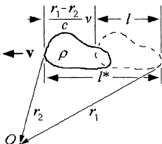
Fig. 3.1 For the two field signals to arrive simultaneously at O, the field signal originating from the leading end of the moving charge must be sent later than the field signal originating from the trailing end of the charge.
