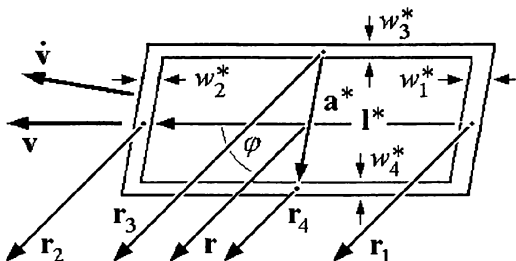
Fig. 4.7 When the charge shown in Fig. 4.6 is in a state of accelerated motion and is at a retarded position, its apparent length, shape, and thickness of its surface layers are no longer the same as for the stationary charge. The distances from the center of the charge and from the four surface layers to the point of observation are represented by the vectors \mathbf{r} , \mathbf{r}_1 , \mathbf{r}_2 , \mathbf{r}_3 , and \mathbf{r}_4 . All five \mathbf{r} 's meet at the point of observation (origin of coordinates). The acceleration vector is in the xy plane.
