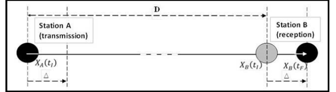
Figure 2. One-way measurement of the velocity of light – eastward transmission
