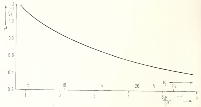
FIGURE 5. Mobility, \mu , as a function of the gate voltage, V_G , and the density of conduction electrons, N , for a Si MOS transistor. Parameters as for Figs. 3 and 4.
