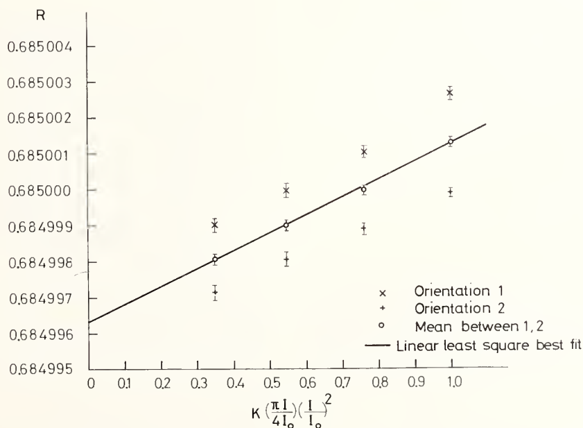
FIGURE 3. Plot of neutron to proton resonance frequencies. The quantity \kappa(\pi I/4I_0)(I/I_0) is an appropriately scaled oscillating power which yields a linear fit. (See references in Ref. [16] for a full description). The two orientations correspond to reversals of the machine axis with respect to the beam velocity.
