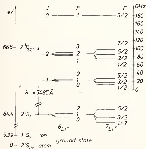
FIGURE 1. Energy level scheme of the 1s2s\ ^3S_1 and 1s2p\ ^3P terms of {}^6,7\text{Li}^+ , the isotope shift is omitted.
