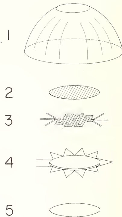
FIGURE 2. Exploded view of the absolute radiometer. 1—hemispherical mirror; 2—black coating; 3—heater; 4—receiver disk with thermocouples; 5—gold coating.
