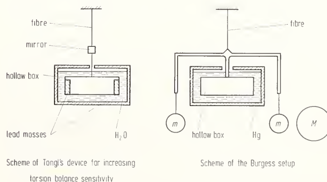
FIGURE 11. Measurement arrangement with buoyancy bearings [58].
