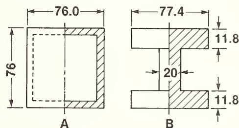
FIGURE 1. Forms of the sinkers A and B (side view). The dimensions are given in mm and they are cylindrical.
