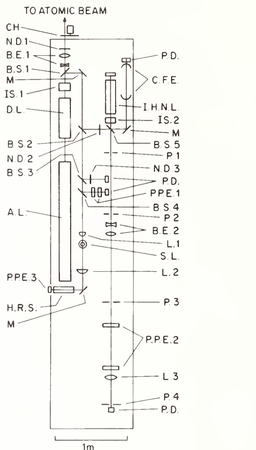
FIGURE 2. Plan of the lasers and optics of the present experiment. CH, chopper; N.D., neutral density filter; B.E., beam expander; M, Mirror; IS, isolator; D.L., dye laser; P.D., photodiode; C.F.E., confocal scanning Fabry-Perot etalon; I.H.N.L., iodine stabilized, ^4\text{He} - ^{22}\text{Ne} laser (primary wavelength standard; plasma tube Jodon CE-16-1.5 CS); A.L., argon ion laser; P.1, P.2, pinholes, 1 mm diameter; P.P.E., plane parallel Fabry-Perot etalon, 1 and 2 pressure scanned; L, Lens; P.3, pinhole, 2-5 mm diameter; P.4, pinhole, 50 \mu\text{m} diameter; S.L., atomic wave length standard lamp; H.R.S., Hartridge reversion spectroscopy.
