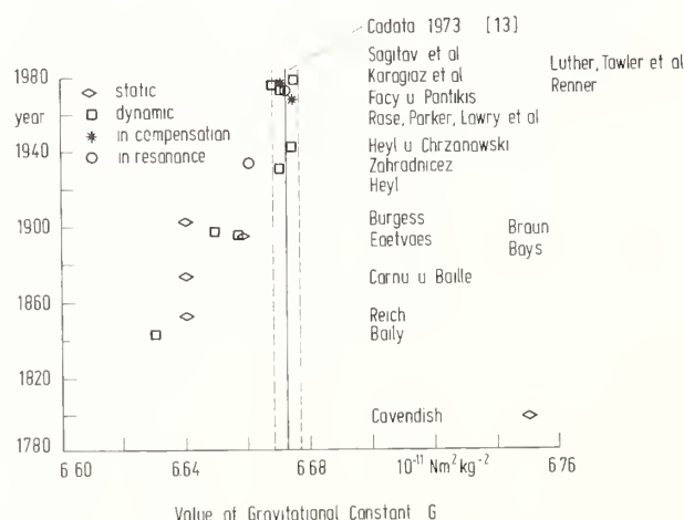
FIGURE 7. Compilation of G values attained by torsion beam balance measurements.
