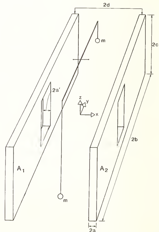
FIGURE 3a. A schematic diagram of the beam balance and its associated masses.
