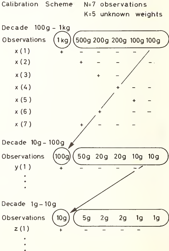
FIGURE 3. Simple calibration scheme with 5 unknown masses (K) and 7 weighings (N).
