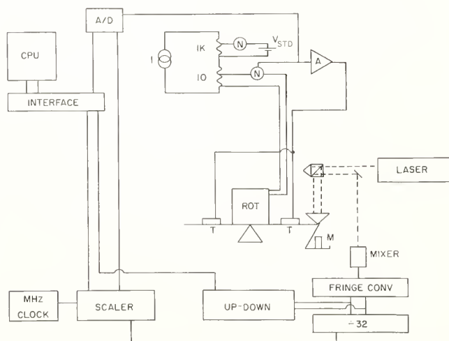
FIGURE 2. Block diagram for voltage integral determination. T: Torquing coils; M: standard mass; ROT: Main rotatable coil; N: Null detectors; A: servo amplifier.
