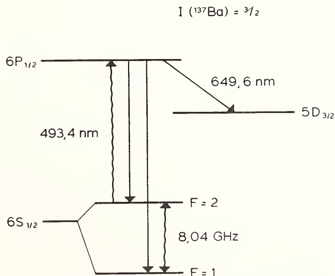
FIGURE 2. Relevant energy levels of \text{Ba}^+ .
