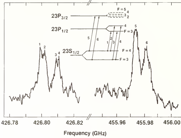
FIGURE 3. Single photon 23S \rightarrow 23P transition in Cs. The large frequency difference (29172 MHz) between the two groups "1-2-3-4" and "5-6" is due to the fine structure 23P_{1/2} - 23P_{3/2} of the 23P level. Also observed are: the hyperfine structure of the 23S_{1/2} level (9.2 MHz) in the separation "5" to "6" and "1-2" to "3-4", and the hyperfine structure of the 23P_{1/2} level on the splitting (2.2 MHz) "1" to "2" and "3" to "4". The hyperfine structure of 23P_{3/2} is unresolved here.
