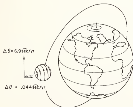
FIGURE 1. Relativistic precessions: Geodetic and motional.
