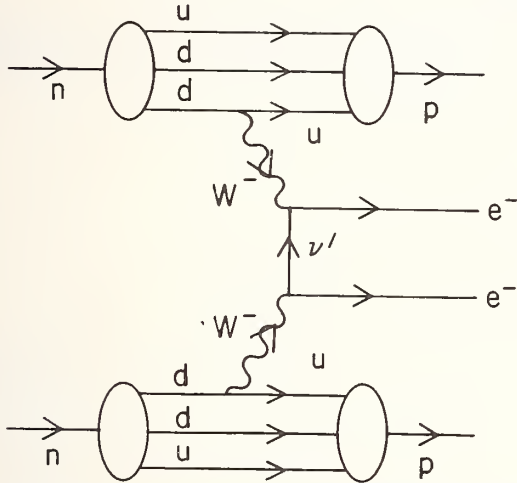
FIGURE 13. Diagram leading to double β-decay in nuclei.
