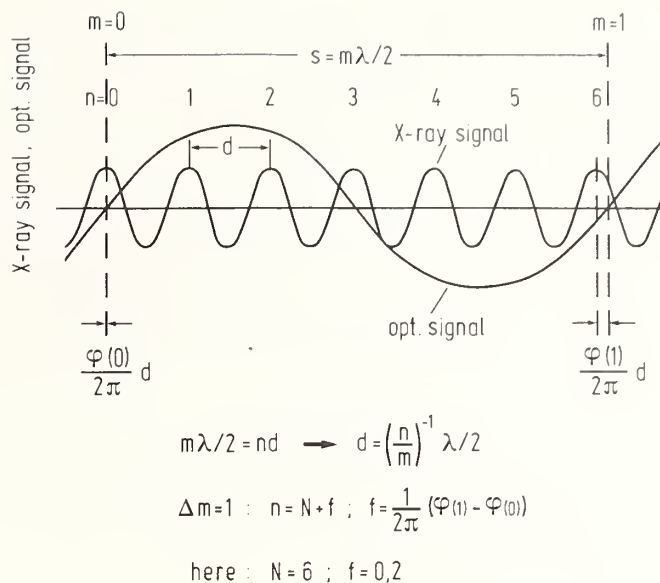
FIGURE 4. Signals obtained in the scanning x-ray interferometer of Fig. 3 (schematically); modulation of the x-ray signal shown, average intensity subtracted.
