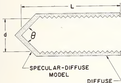
FIGURE 3. Schematic of a cylindrical cavity with a conical bottom. The cylindrical surface is diffuse and the conical surface is intermediate between specular and diffuse.
