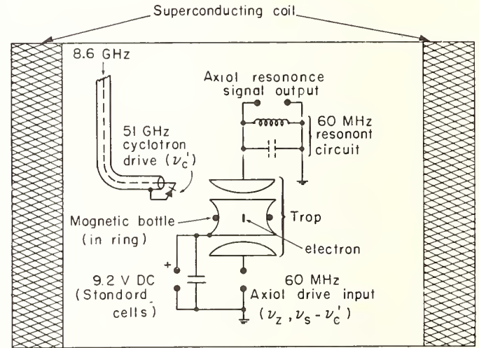
FIGURE 2. Schematic of the University of Washington apparatus used to measure the electron anomaly. This apparatus allows the measurement of the cyclotron frequency \nu_C and the spin-cyclotron beat ( g-2 ) frequency \nu_D = \nu_S - \nu_C on a single electron stored in a Penning trap at \sim 4 K.
