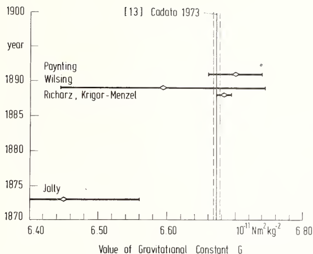
FIGURE 5. Compilation of G values attained by Jolly beam balance measurements.
