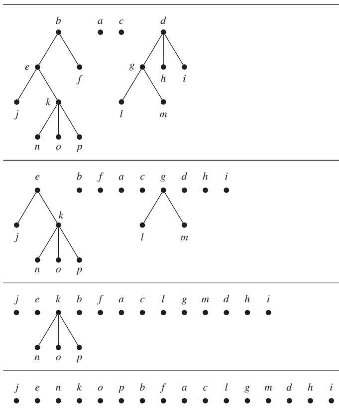
FIGURE 6 The inorder traversal of T .
