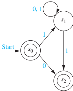
FIGURE 4 A nondeterministic finite-state automaton recognizing L(G) .
