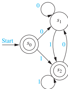
FIGURE 5 A finite-state automaton.
