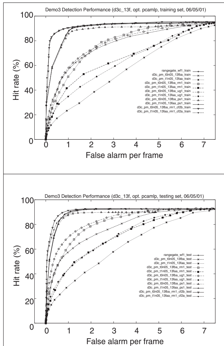
Figure 14. Performance curves.
