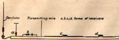
Illustrating Typical Arrangements for Collecting Energy in a System of Transmission Thru a Single Wire. Fig. 5.
