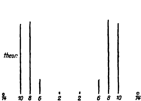
FIG. 3.— H_\beta \parallel -components.
