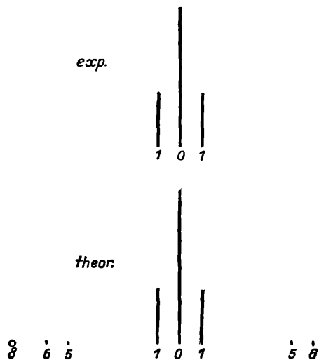
FIG. 2.— H_\alpha \perp -components
