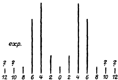
FIG. 2.— H_\alpha \perp -components
