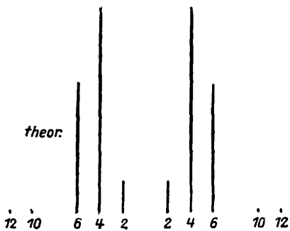
FIG. 4.— H_\beta \perp -components.
