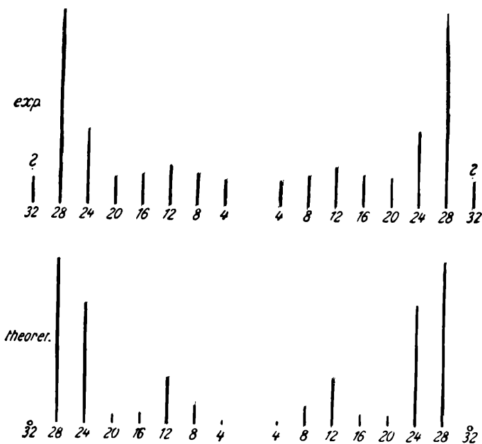
FIG. 7.— H_\delta \parallel -components.
