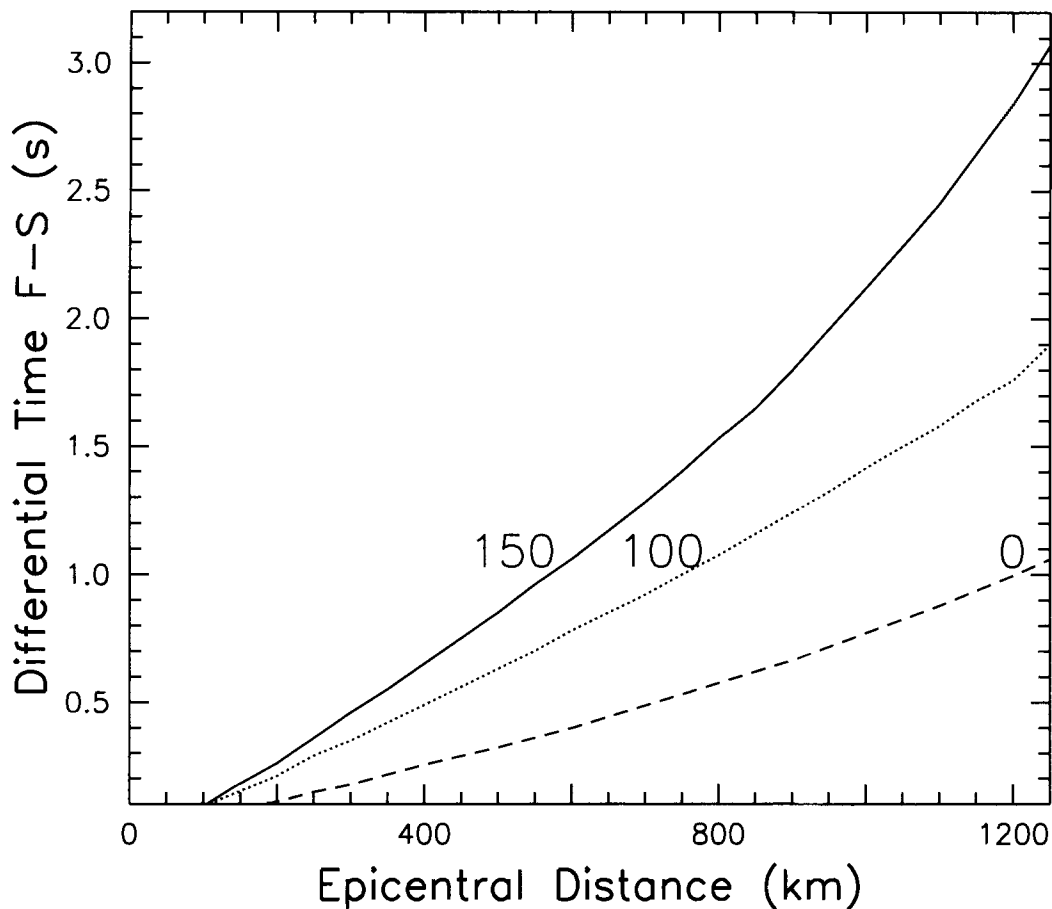
▲ Figure 1. Differential travel time versus epicentral distance for three focal depths starting at an epicentral distance for which the time differential is 0.1 s. The differential travel time is defined as the flat-earth travel time minus the spherical-earth travel time for the P wave based on the iasp91 velocity model. The curves are labeled by the focal depths in kilometers. For other crustal focal depths, the curves are almost identical to that shown for a surface focus, as it is only in the head-wave (flat earth) and P_n (spherical earth) parts of the ray path that the differences become nonnegligible. In the mantle, the differential travel times increase with focal depth for fixed epicentral distance.
