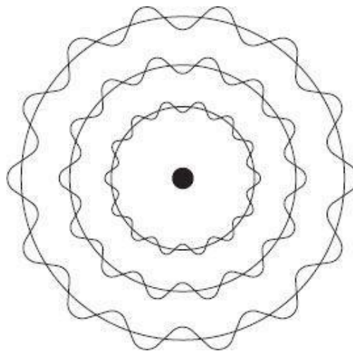
Figure 10: Standing electron waves in the quantum atom
