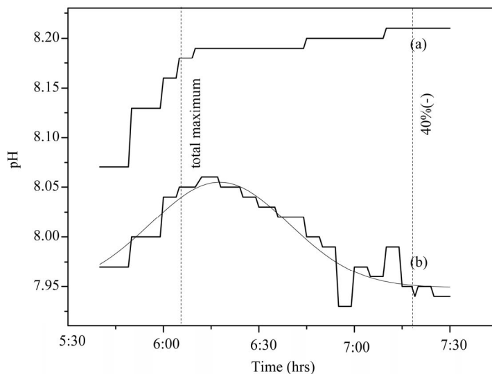
Figure 1. Comparison of solar radiation induced H^+ ion activity in seawater during (a) normal day and (b) partial solar eclipse event on 22 July 2009. The reduction in pH value during eclipse is around 20% of the difference between the ordinary water (pH 7.5) and seawater (pH 8.5). The vertical dotted line is the time of maximum eclipse occurrence, at which the ionisation of seawater started due to the shorter wavelength rays reaching the earth's surface.
