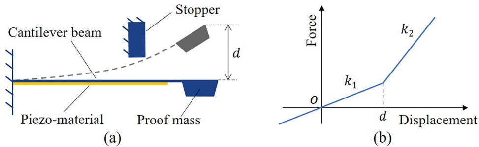
Fig. 12. A nonlinear PEH with a mechanical stopper [87] (contact aided CM [81]). (a) Schematic structure. (b) Piecewise-linear stiffness ratio.
