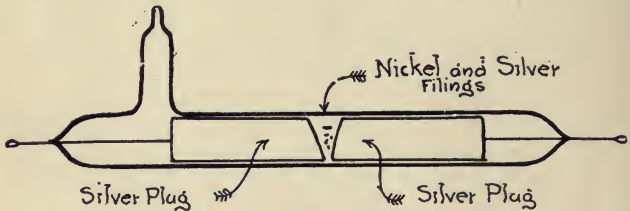
FIG. 84.—Marconi coherer.
