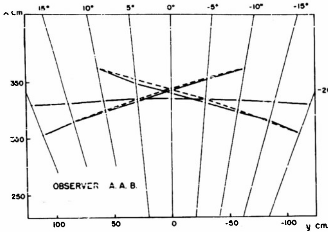
Fig. 19. Frontal and Oblique Geodesics. Solid lines show experimental settings. Dotted lines show prediction of oblique settings computed from frontal settings.
