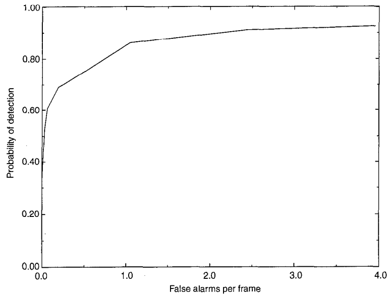
Figure 1. ROC curve on Hunter Liggett April 1992 imagery. Horizontal axis gives average number of false alarms per frame. Vertical axis is target-detection probability.
