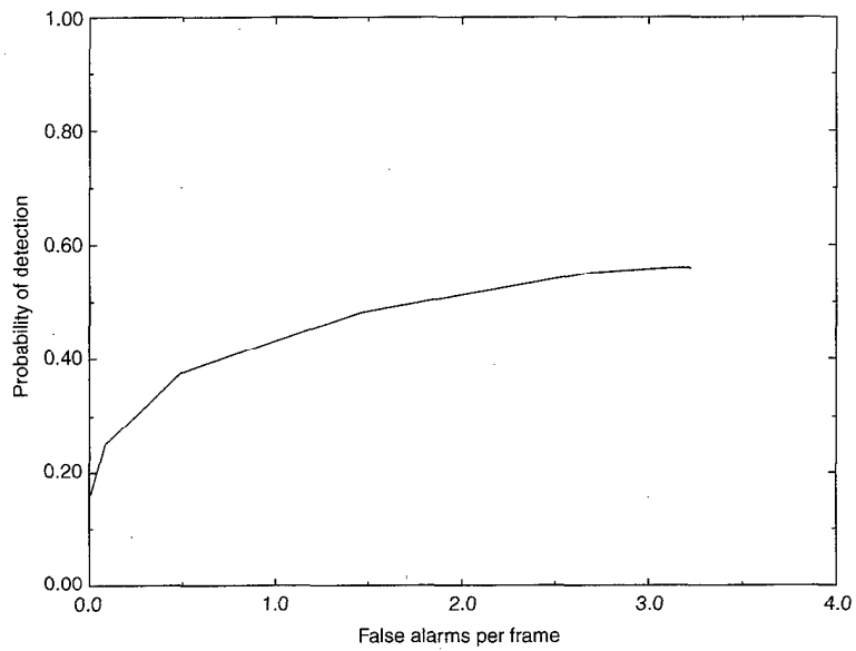
Figure 2. ROC curve on Yuma July 1992 imagery.
