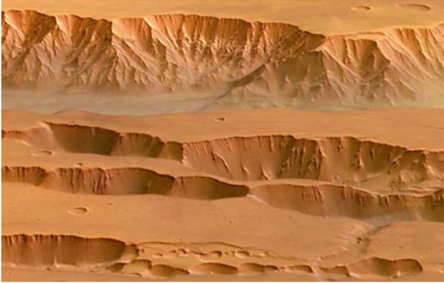
FIG. 15.19 : Oblique view of Coprates Chasma, the eastern part of Valles Marineris. The canyon is 8 km deep. Image acquired by the High Resolution Stereo Camera (HRSC) aboard Mars Express, on 28 May 2005. Credit: ESA, DLR, FU Berlin (G. Neukum).
