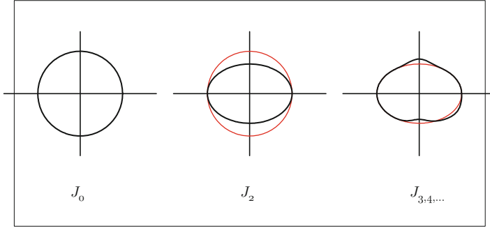
FIG. 3.2 : Changing perception of the shape of the Earth in geodesy. Left: Sphere, with C_{00} = -J_0 = 1 and J_1 = 0 . Center: From the sphere to the ellipsoid of revolution, with J_2 term indicating flattening. Right: From the ellipsoid to the geoid, with J_n terms n \geq 3 .
