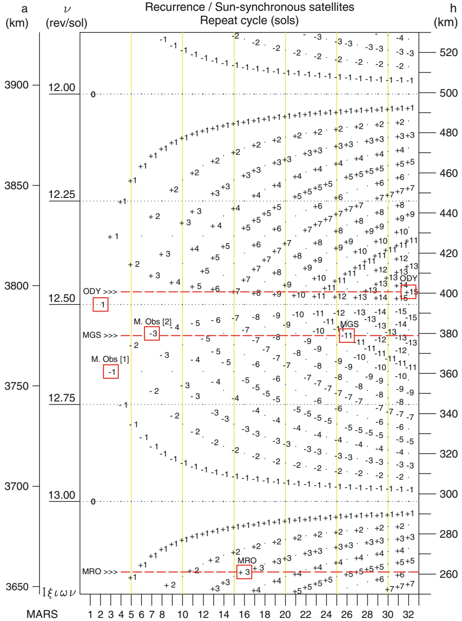
FIG. 15.28 : Recurrence diagram for Sun-synchronous satellites. For altitudes between 250 and 530 km, the possible recurrence cycles are indicated by the value of D_{T_o} . Boxed values correspond to the exact recurrence cycles appearing in Table 15.6, or to approximate, but shorter cycles determined in Example 15.7. For example, for Mars Odyssey (ODY), we have the triple [12, +1, 2] , or \nu_o = 12 (the integer closest to \nu , as ordinate), D_{T_o} = +1 (indicated on the diagram), and C_{T_o} = 2 (as abscissa).
