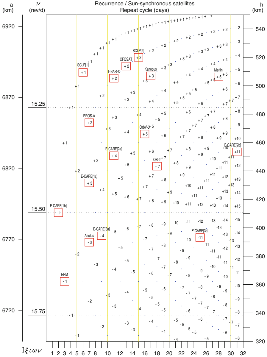
FIG. 11.3: Recurrence diagram for Sun-synchronous satellites. For altitudes between 320 and 540 km, possible recurrences are indicated by specifying D_{T_o} . Boxed values correspond to satellites appearing in Tables 11.1 and 11.3. For example, for TerraSAR-X, we have the triple [15, +2, 11] , whence \nu_o = 15 (the integer closest to \nu , as ordinate), D_{T_o} = +2 (indicated on the diagram), and C_{T_o} = 11 (abscissa), 11 day cycle.
