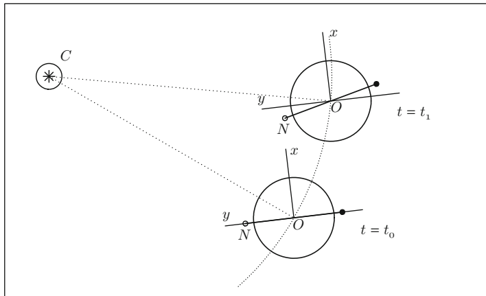
FIG. 10.1 : Position of the line of nodes in the geocentric frame \mathfrak{R} (O; x, y, z) at two times t_0 and t_1 , where C is the center of the Sun, O is the center of the Earth, and Oxy lies in the equatorial plane. The ascending node is denoted by N .
