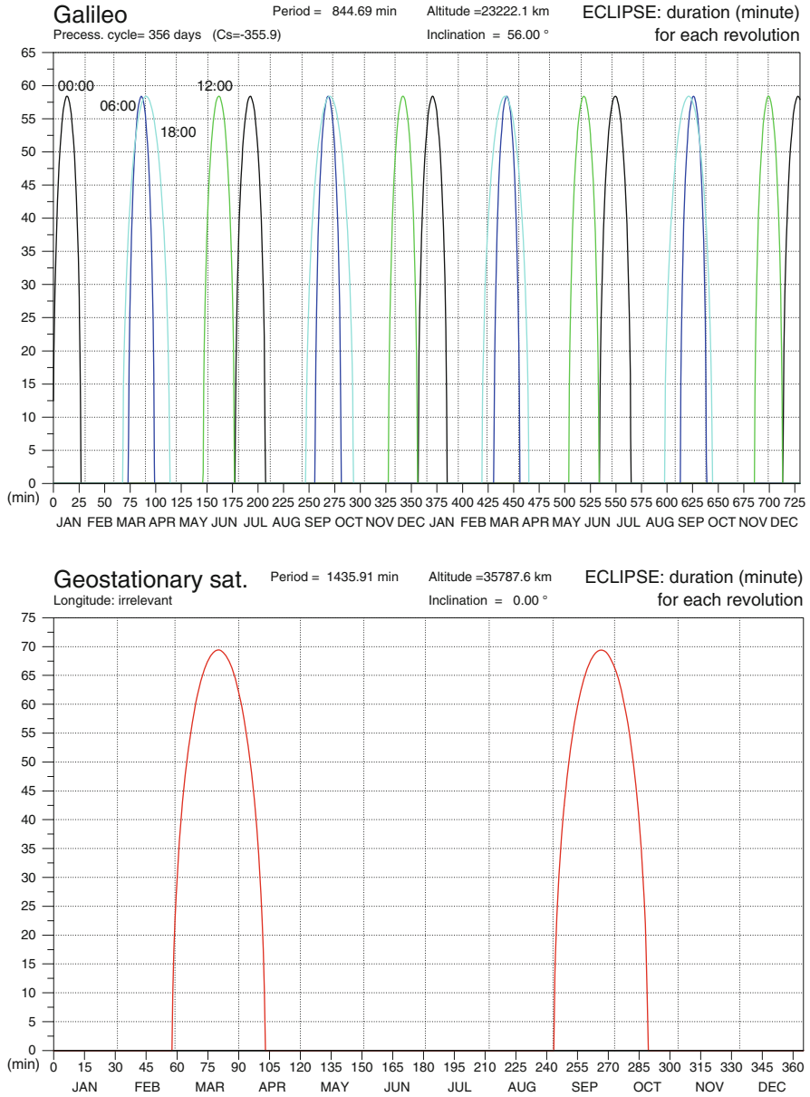
FIG. 10.26 : Length of solar eclipse in minutes as a function of the day of the year. Upper: MEO satellite with four values of the ascending node crossing time (LMT), the initial reference day. Lower: GEO satellite, for any value of the parking longitude.
