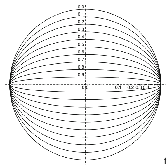
FIG. 1.8: Ellipses with the same semi-major axis but flattening f varying from 0.0 to 0.9, in constant steps of 0.1. The corresponding flattening f is indicated on one of the two foci and on one end of the semi-minor axis. Note that the ends of the semi-minor axes are regularly spaced.
