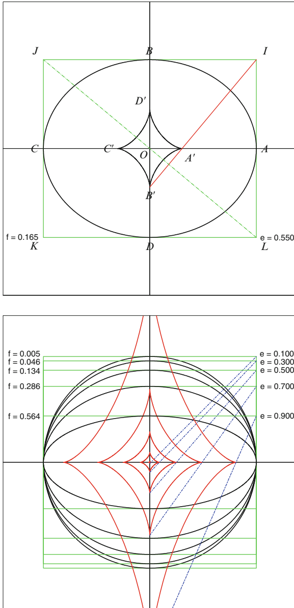
FIG. 1.12 : Relationship between an ellipse and its evolute. Upper: The straight line joining A' and B' , centers of curvature for A and B , respectively, passes through I and is perpendicular to the diagonal JL of the rectangle IJKL , a rectangle with sides 2a and 2b , center O , escribed on the ellipse. Lower: The same construction for different values of the eccentricity between e = 0.10 and e = 0.90 , in steps of 0.20 . The semi-major axis remains constant.
