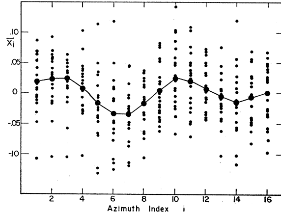
FIG. 2. The individual column means \bar{x}_i are plotted as a function of azimuth position for the July, 1925 observational data. Large circles and the connecting curve show the second harmonic effect exhibited by the averages, \langle \bar{x}_i \rangle , due to ordering in azimuth. Units for the ordinate are fringes.
