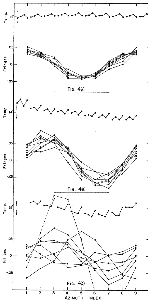
FIG. 4. The temperature pattern in the observation hut and the observed fringe shift is shown here for three dates: Fig. 4(A), August 30, 1927 (Cleveland); 4(B), September 23, 1925 (Mount Wilson); 4(C), July 30, 1925 (Mount Wilson). Each group of four points in the upper parts of the figures represents the thermometer readings on the four walls of the hut at a given time between midnight and dawn (a range of about 5 hours in sidereal time). Arrows at the left of the temperature scales indicate a 1^\circ range. The lower part of each figure shows the fringe shift as a function of azimuth index for the times corresponding to the temperature patterns. The lower part of each figure shows the fringe shift as a function of azimuth index for the times corresponding to the temperature patterns. The dashed curve in Fig. 4(C) shows the fringe displacement when direct sunlight fell on the interferometer at dawn.
