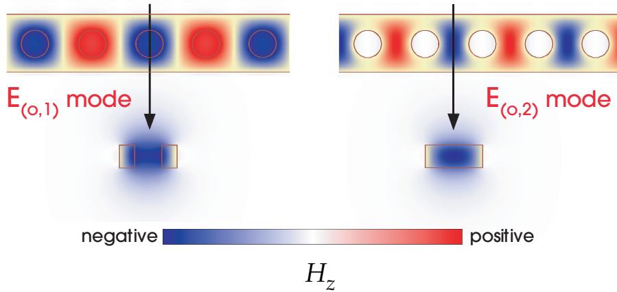
Figure 6: Cross sections of H_z field for lowest-order TE-like modes from figure 5 at the Brillouin-zone edge, k = \pi/a . Left: first band (lower edge of gap). Right: second band (upper edge of gap). The upper plot shows the z = 0 horizontal cross sections, in which H_z is the only magnetic-field component. The lower plots show x cross sections at the positions indicated by the arrows (through the H_z peaks). The dielectric material is shown as translucent yellow shading.
