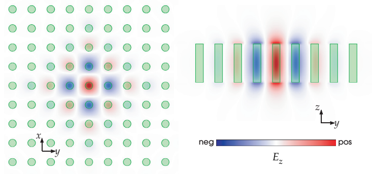
Figure 12: E_z cross sections for resonant “monopole” mode of a point defect in the rod slab (dielectric material shown as translucent green), formed by reducing the dielectric constant of the center rod and its four nearest neighbors from \epsilon = 12 to \epsilon = 9 . The mode decays exponentially in the plane of the slab, but slowly radiates away vertically.
