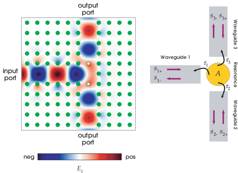
Figure 7: Left: E_z field in “T” splitter for waveguide of figure 2, showing essentially 100% transmission (50% in each branch) at \omega a / 2\pi c \approx 0.4 . Right: Abstract model, treating junction as weak resonance, predicting 100% transmission when 1/\tau_1 = 1/\tau_2 + 1/\tau_3 . Thus, to get 100% transmission, we cannot use a symmetric junction, and must insert rods (white rods with \epsilon = 3.5 ) that obstruct the output waveguides in order to increase transmission.
