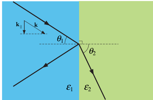
Figure 4: For a flat interface between two dielectrics \epsilon_1 and \epsilon_2 , light can be described by a ray with an incident angle \theta_1 and a refracted angle \theta_2 given by Snell's law. When \epsilon_2 < \epsilon_1 , we can have no solution \theta_2 for certain \theta_1 , and the light undergoes total internal reflection. A generalization of this result follows from translational symmetry, which tells us that k_{\parallel} is conserved.
