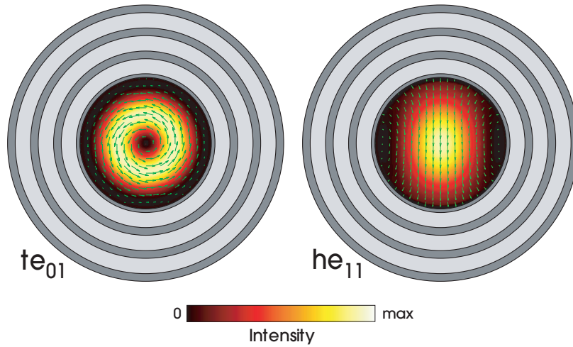
Figure 16: Intensity patterns for two core-guided modes in hollow-core Bragg fiber of figure 15 at the quarter-wave frequency. Power intensity is shown by color scale, and transverse ( xy ) electric-field pattern is shown by green arrows.
