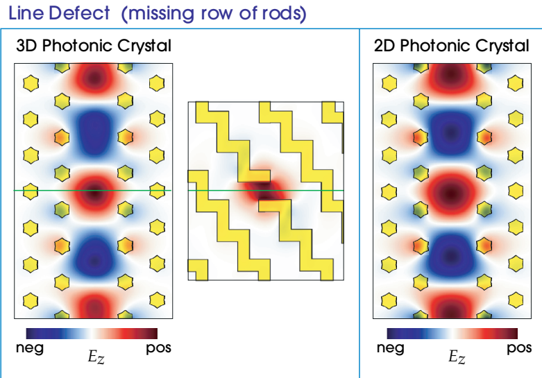
Figure 17: Horizontal and vertical cross sections (intersecting at green lines) of E_z field patterns of a linear defect in the layered structure (left), formed by removing a row of rods from a single rod layer, compared to the field for the corresponding TM state in a two-dimensional crystal (right) with the same rod cross section. These fields correspond to a wave vector k_x \tilde{a} / 2\pi = 0.3 along the waveguide, where \tilde{a} is the in-plane lattice constant from figure 12. Dielectric material is shown in yellow.
