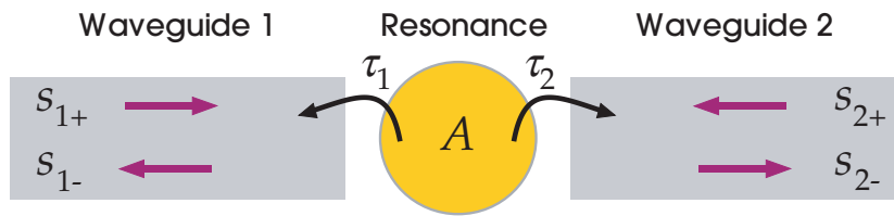
Figure 5: Abstract diagram showing the essential features of the filter from figure 4: a single-mode input waveguide 1, with input/output field amplitudes s_{1+}/s_{1-} ; a single-mode output waveguide 2 with input/output field amplitudes s_{2+}/s_{2-} ; and a single resonant mode of field amplitude A and frequency \omega_0 , coupled to waveguides 1 and 2 with lifetimes \tau_1 and \tau_2 ( \tau_1 = \tau_2 in figure 4). The s_{\ell\pm} are normalized so that |s_{\ell\pm}|^2 is power in the waveguide, and A is normalized so that |A|^2 is energy in the cavity.
