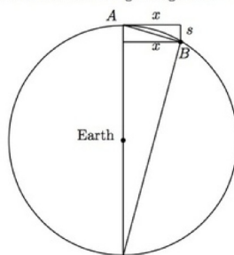
FIGURE 1. The moon starts at A. In one second it moves to B, falling a distance s while moving horizontally a distance x . The diameter of the orbit is D so the vertical side of the big triangle is D - s .
