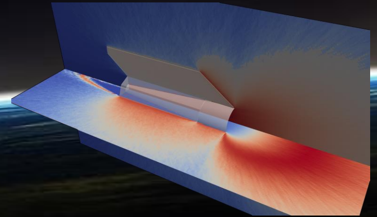
Particle-simulation
