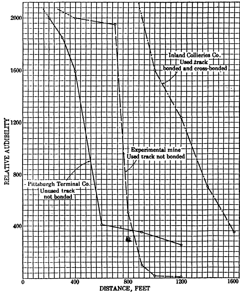
FIGURE 20.—Transmission along car rails
