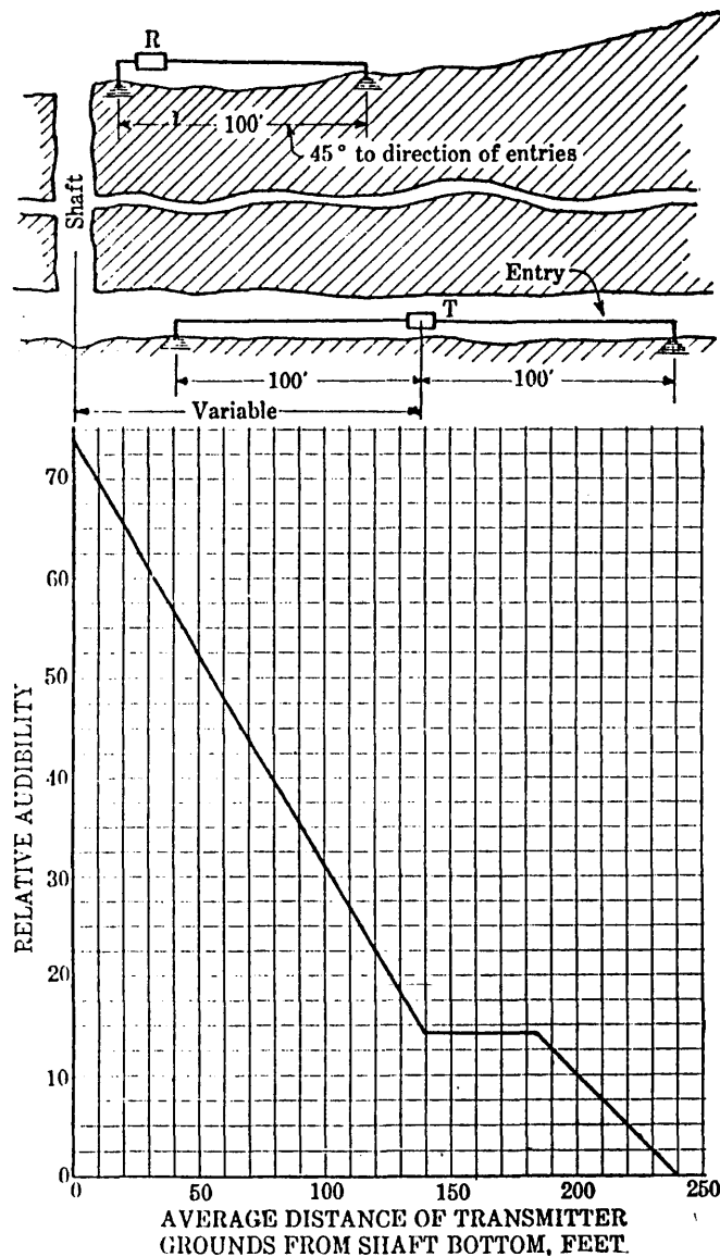
FIGURE 25.—Effect on audibility of increasing distance between transmitting and receiving stations
