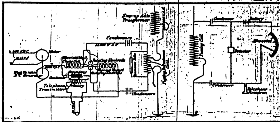
The Elements of the Collins Wireless Telephone System and Their Electrical Relation to One Another.
