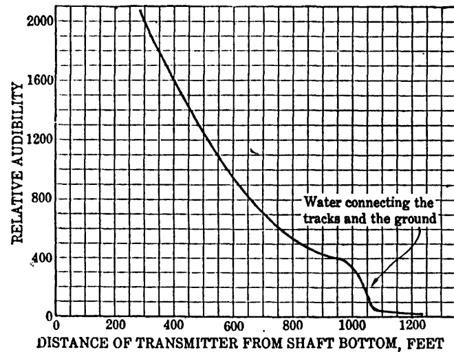
FIGURE 22.—Decrease in audibility with increase in distance from receiving station. (Modified track transmission, see fig. 14, B)
