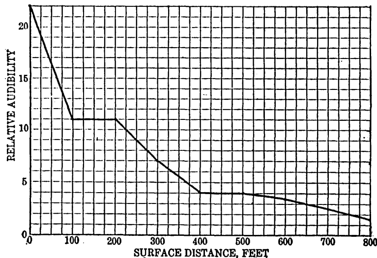
FIGURE 23.—Decrease in audibility with distance from transmitter
