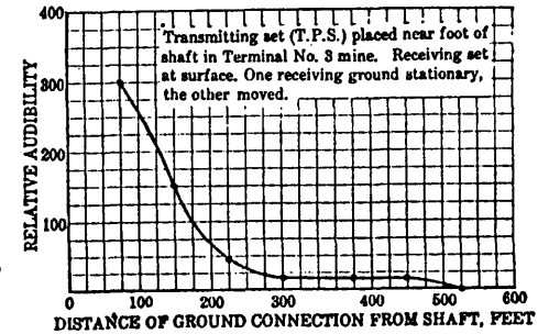
FIGURE 26.—Relation between audibility and distance between receiving grounds
