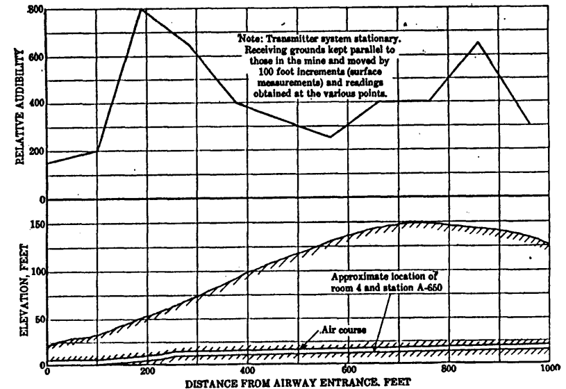
FIGURE 24.—Transmitting T. P. S. signals from inside experimental mine through overburden
