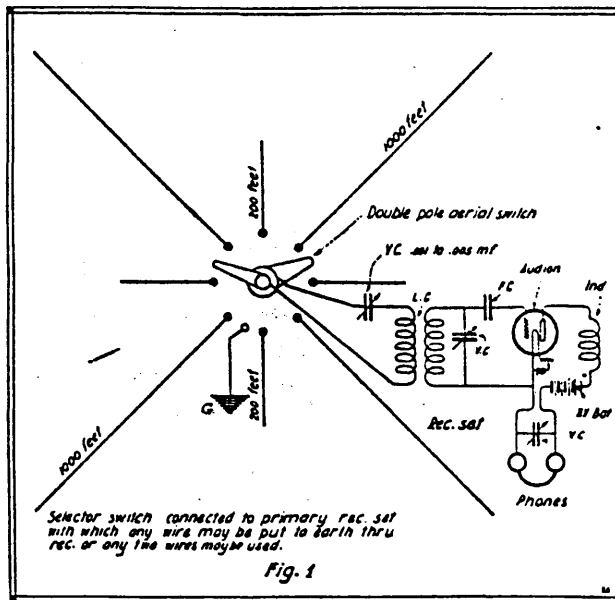
Rogers Underground Aerial System for General Requirements, Showing Bipolar Selector Switch Connected to Primary Circuit of Receiving Set. Any Aerial Wire May Be Grounded Thru the "Set," or Any Two Wires May Be Used as Desired.
