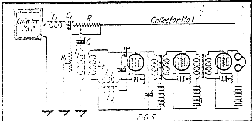
This Circuit Shows an Arrangement for Balancing the Land, Collector No. 2, Which Serves as a substitute for the "Land" Wire Balanced Against the "Sea" Wire, as Shown in the Previous Circuits. Notice That the "Sea" Wire is Shunted Through a Resistance R , Which Was Found Very Important. The Resistance R is Sufficiently High to Give the Loop 2 a Very High Q-factor.
