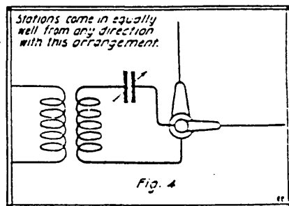
With This Arrangement the Signals Came in Equally Well from Any Direction. A Good "Stand-by" Hook-up.
