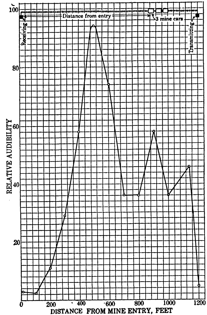
FIGURE 21.—Effect of mine cars on transmission along car rails
