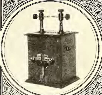
Fig. 2. Small Tesla Coil for gas engine ignition and similar uses
