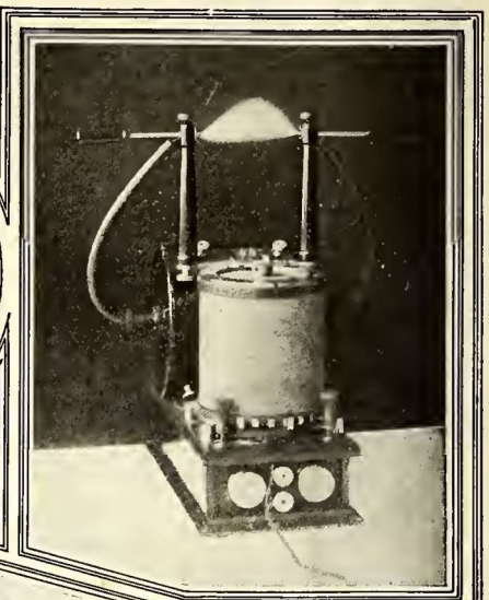
Fig. 4. Tesla Oscillator in action, generating undamped waves
